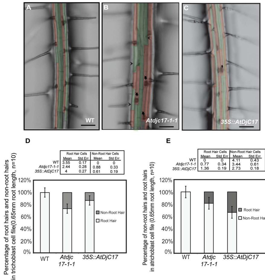
FIGURE 1 | Trichoblast and atrichoblast cells are arranged randomly in AtdjC17 and overexpressor mutants. (A–C) False colored stereomicroscope images of wild-type (WT; A ), AtdjC17-1-1 ( B ) and 35S::AtDjC17 ( C ) illustrate the patterning of root hair cells (red) and non-root hair cells (green) in cell files. Stars represent ectopic root
