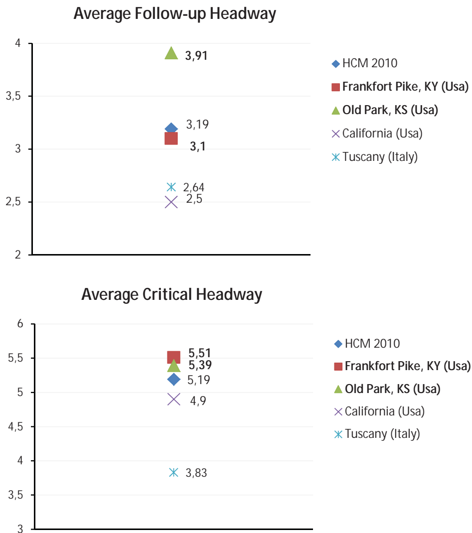
Figure 6: Estimates of critical and follow-up headway for two US locations.
