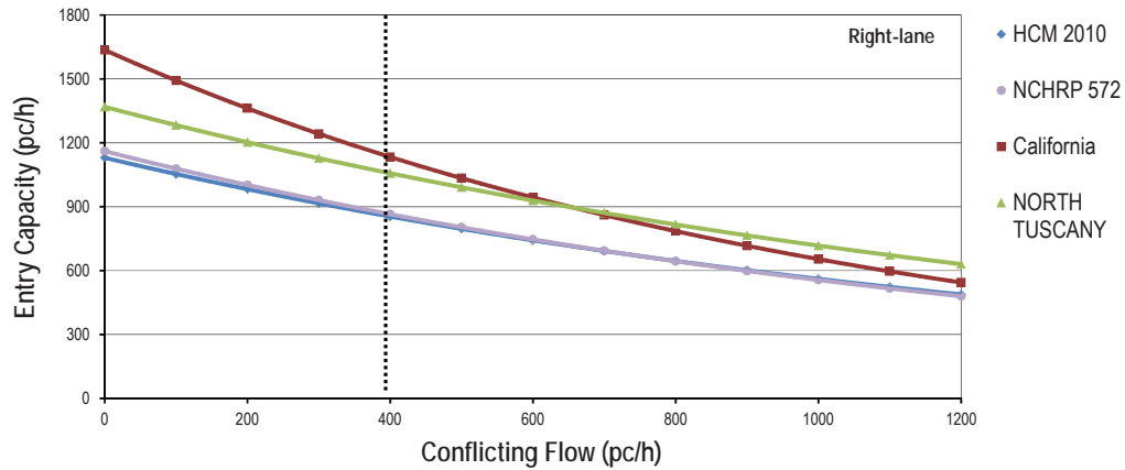
Figure 4: HCM 2010 roundabout capacity model calibration: right lane.
