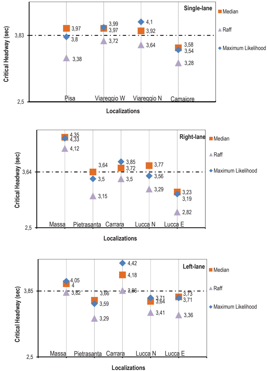
Figure 2: Results for each estimation method: comparison.
