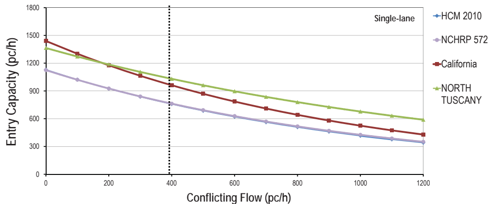
Figure 3: HCM 2010 roundabout capacity model calibration: single lane.
