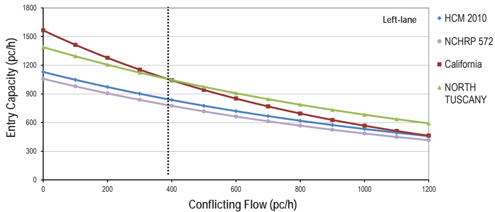
Figure 5: HCM 2010 roundabout capacity model calibration: left lane.
