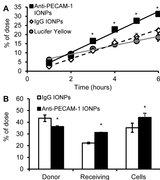
Figure 5. Anti-PECAM-1 IONP flux across hCMEC/D3 cells and cell association results. Anti-PECAM-1 IONP (0.05 mg/ml), IgG IONP (0.05 mg/ml) and LY (100 µM) flux across hCMEC/D3 cells for 6 h (A). Anti-PECAM-1 IONP and IgG IONP distribution in the donor and receiving chambers and hCMEC/D3 cells at 6 h (B). (N=3, mean ± SD) * Significantly different compared to IgG IONPs. doi:10.1371/journal.pone.0081051.g005
