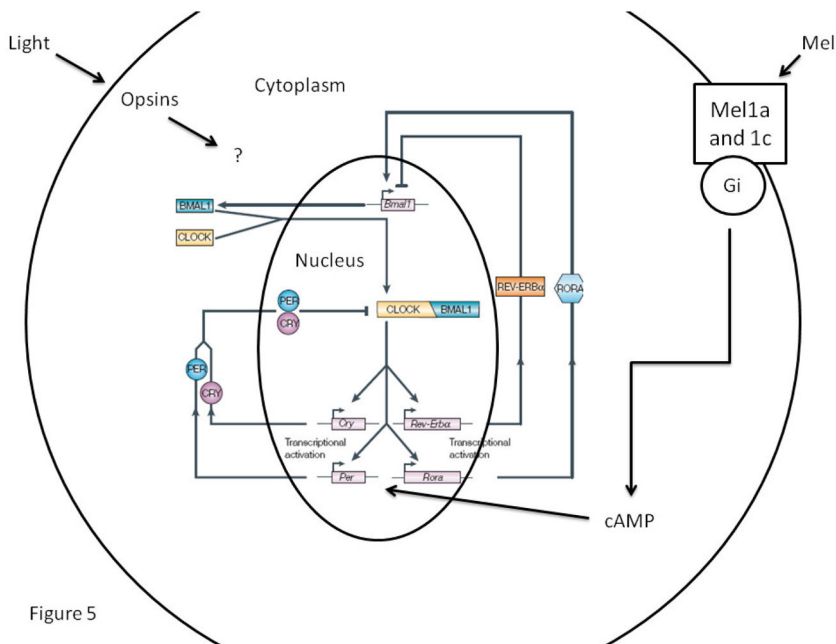
Figure 5. Schematic of the regulatory loops of clock genes in the vertebrate cell. Perhaps, melatonin influences this process through its receptors that are linked to Gi GTP proteins. By decreasing cellular cAMP levels, melatonin may modestly alter period expression, whose promoter contains a CRE but several “E-boxes” (modified from Bell-Pedersen et al. 2005 with permission).
