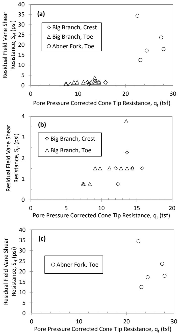
Figure 5.40: Correlations between the residual field vane shear resistance, S_{rf} , and the corrected cone tip resistance, q_t , at (a) both impoundments, (b) Big Branch and (c) Abner Fork.
