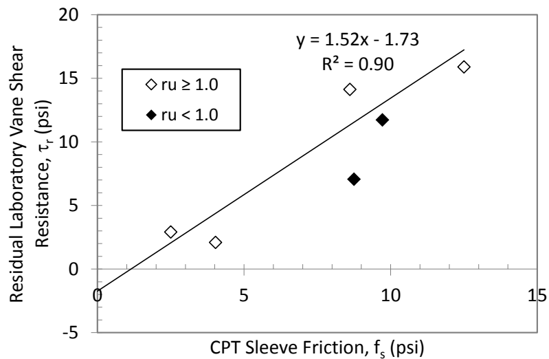
Figure 5.61: Correlation between the residual laboratory vane shear strength and the CPT sleeve friction for samples with PI > 7.0%.
