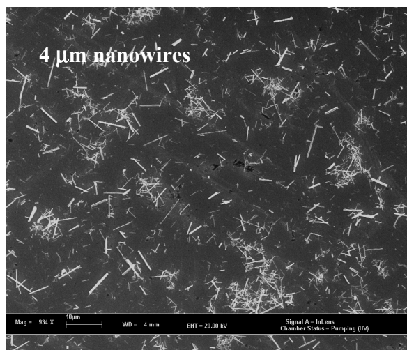
Figure 4.1.b. SEM images of aggregates of “single” \text{WO}_3 nanowires after 5 minutes, 20 minutes, and 1 hour of ultrasonication (10, 6, and 4 \mu\text{m} average length, respectively).
