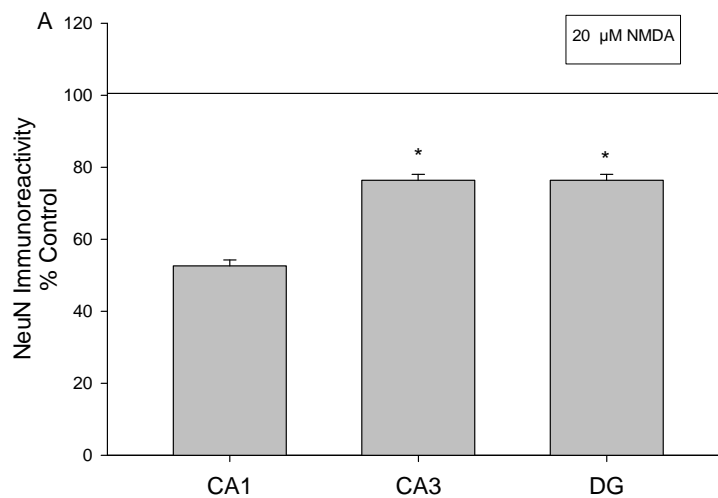
Figure 3: Effects of exposure to 20 \mu\text{M} NMDA on NeuN immunofluorescence in the pyramidal cells of the CA1 as compared to the pyramidal cells of the CA3 and the granule cells of the DG (* p< .05 vs. CA1).
