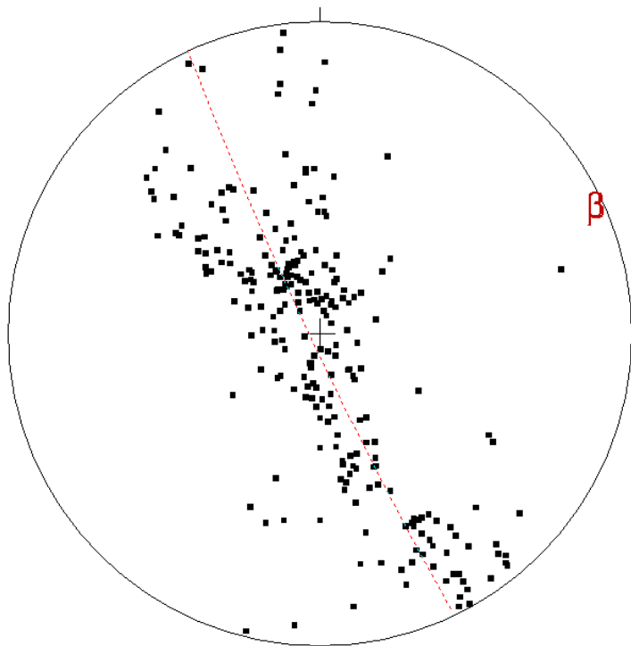
Figure 4-10 Equal-area stereonet plot of poles to bedding on Simms Mountain-Horseleg Mountain fold train
