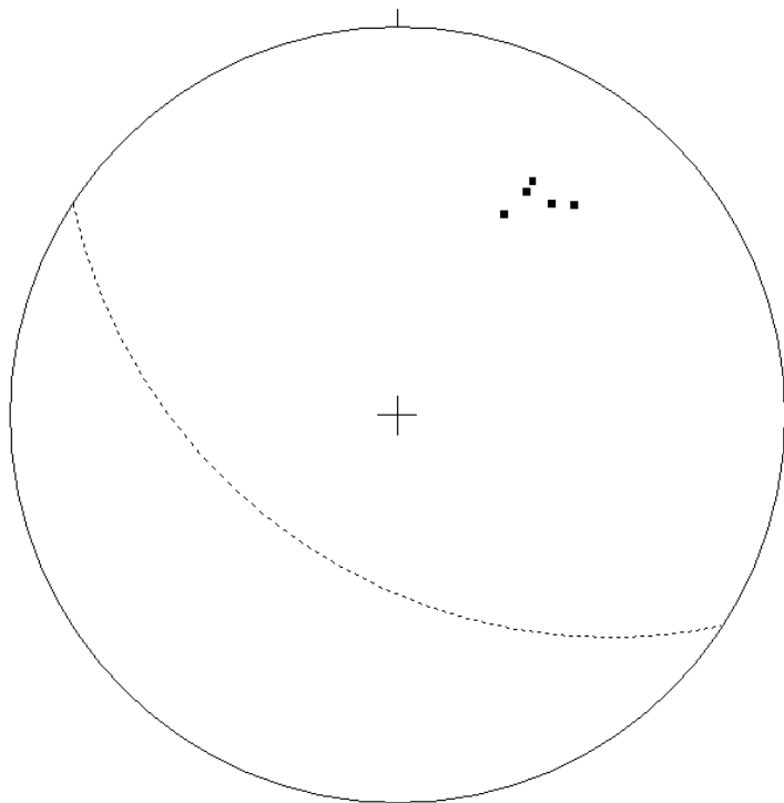
Figure 4-4 Equal-area stereonet plot of poles to bedding on Taylor Ridge monocline small-scale fold
