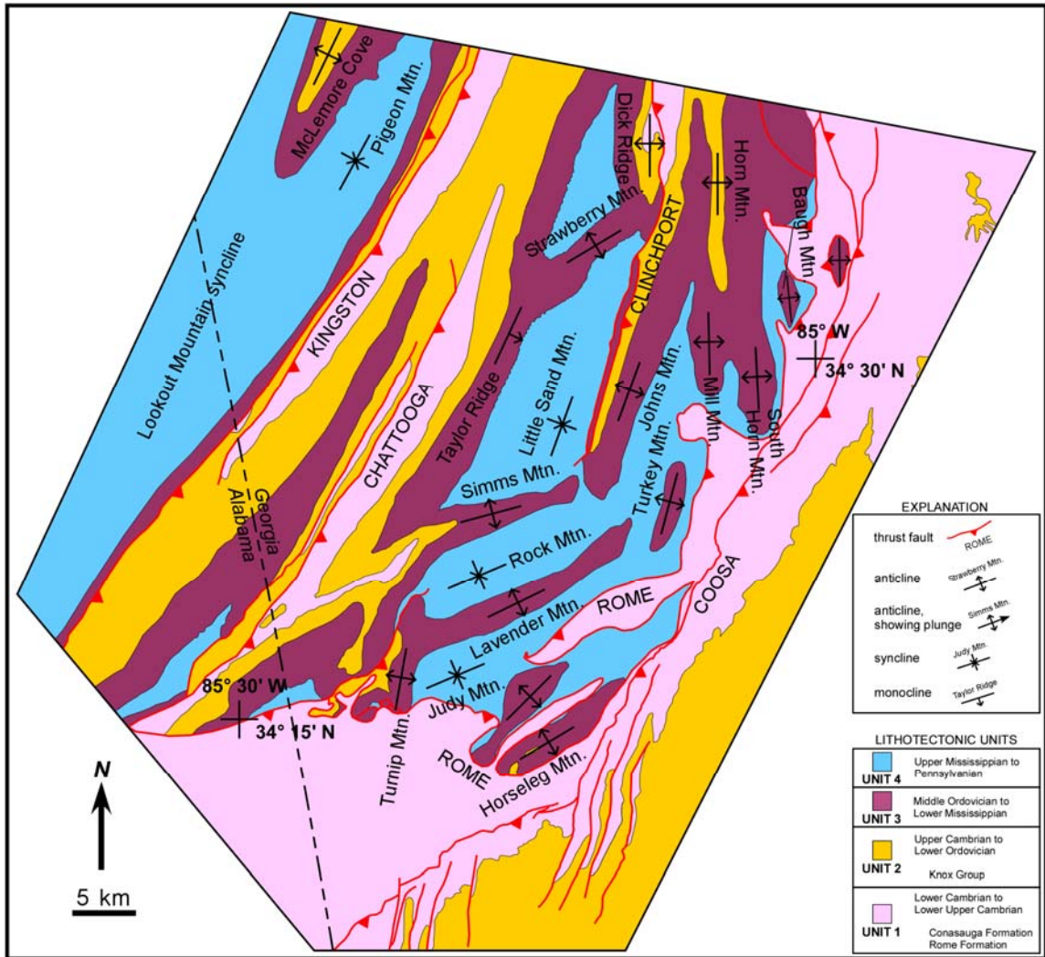
Figure 1-4. Geologic map of the subrecess in Georgia, compiled from field data of the author, as well as Butts (1948), Cressler (1963, 1964a, b, 1970, 1974); Georgia Geological Survey (1976), Thomas and Cramer (1979), Osborne et al. (1988), and Thomas and Bayona (2005). Plunge directions of fold hinges are denoted by closed arrows and the major folds are labeled. Fault names are in all-capital letters. The Kingston–Chattooga anticlinorium is the structurally high outcrop area dominantly of Units 1 and 2 between Lookout Mountain syncline and Taylor Ridge monocline. The Floyd synclinorium (including Little Sand Mountain, Rock Mountain, and Judy Mountain synclines, as well as other unnamed folds) encompasses the entire outcrop area of Unit 4 southeast of the Kingston and Chattooga faults.
