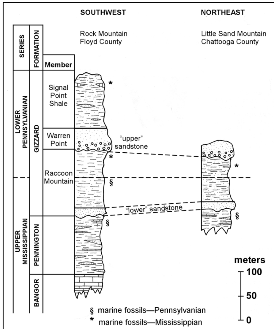
Figure 3-11. Details of biostratigraphic markers in the Lower Pennsylvanian and Upper Mississippian, adapted from Crawford (1989).
