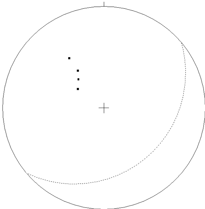
Figure 4-20 Equal-area stereoplot of poles to bedding on Taylor Ridge monocline west of intersection with Strawberry Mountain anticline
