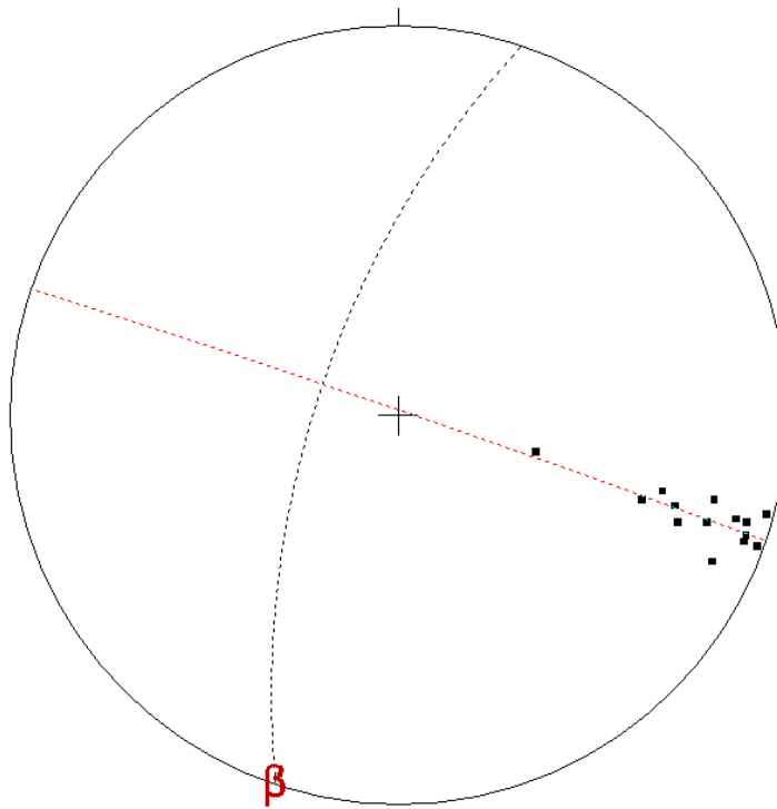
Figure 4-7 Equal-area stereonet of poles to bedding on Dick Ridge anticline
