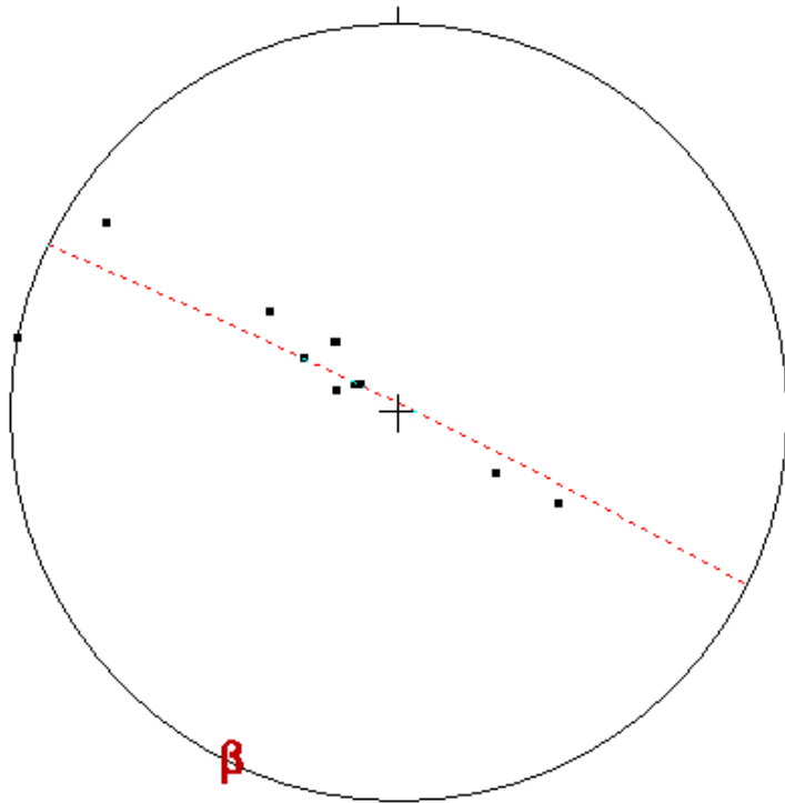
Figure 4-9 Equal-area stereonet plot of poles to bedding on Turkey Mountain anticline
