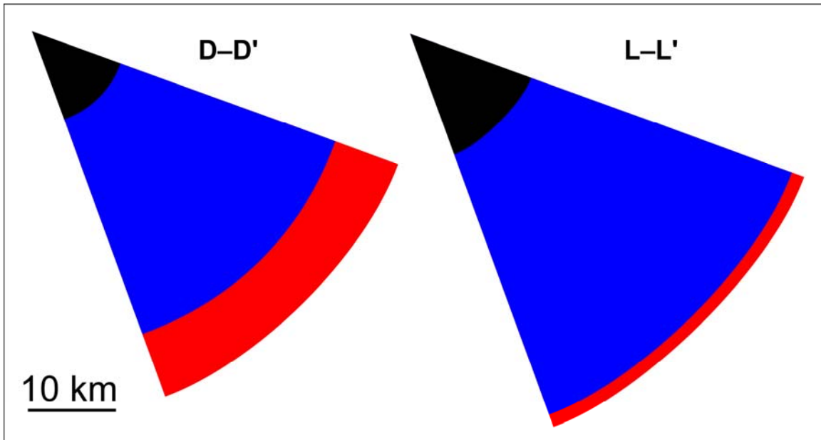
Figure 5-10. Calculations made from actual measurements on cross sections D–D' and L–L' in an attempt to compare results with the simplistic model in Figure 2-2. The area shown in black is a projection of the distance along each cross section between the intersection of the cross sections to the hinge of Taylor Ridge monocline. The area shown in blue is a projection of the deformed-state line length between the hinge of Taylor Ridge monocline to the trailing edge of the fold train through which the cross section is drawn. The area shown in red is the projection of the difference between the restored-state line length between the hinge of Taylor Ridge monocline to the trailing edge of the fold train through which the cross section is drawn and that same line-length in the deformed state.
