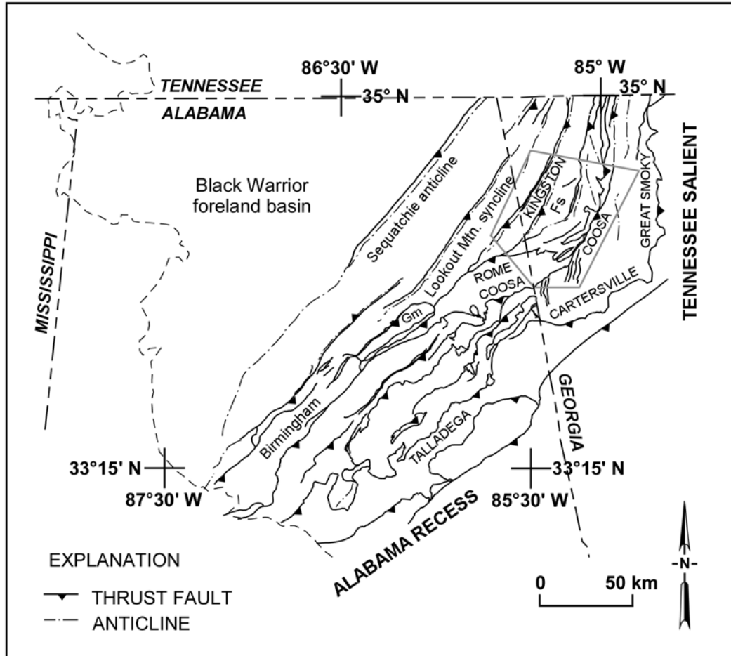
Figure 1-3. Structural outline map of the Appalachian thrust belt in Alabama and Georgia, adapted from Thomas (2007). The gray polygon shows the location of the more detailed map in Figure 1-4. Names of faults are in all capital letters. The Floyd synclinorium is labeled as Fs, Gadsden mushwad as Gm. The label “Birmingham” shows the location of both the surface thin-skinned Birmingham anticlinorium and the subsurface Birmingham basement graben.
