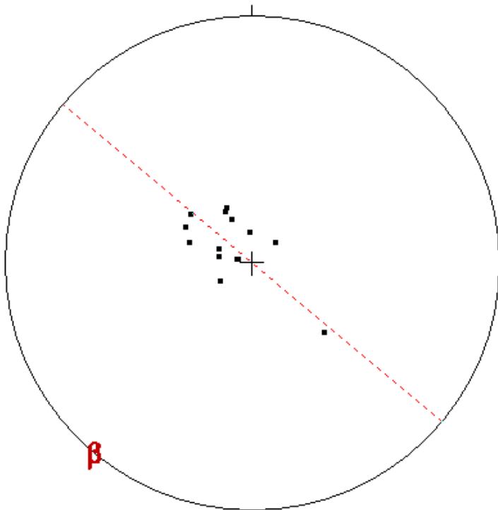
Figure 4-6 Equal-area stereoplot of poles to bedding on Little Sand Mountain syncline
