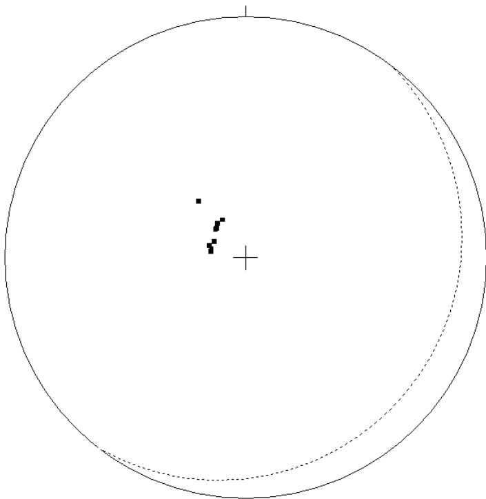
Figure 4-22 Equal-area stereonet plot of poles to bedding on Taylor Ridge monocline south of intersection with Strawberry Mountain anticline
