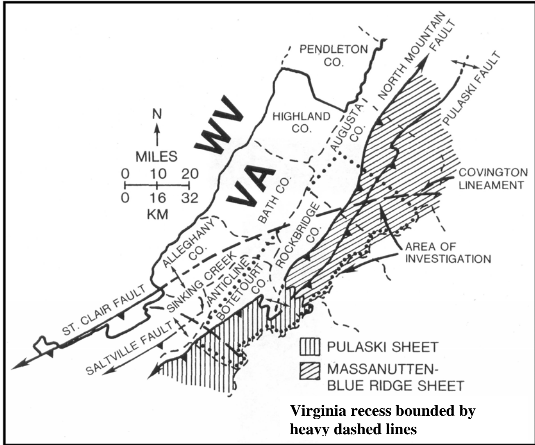
Figure 2- 4. Location map of the abrupt bend in the Appalachian thrust belt of central western Virginia and major structural features, from Kulander and Dean (1988). Note the composite Pulaski/Massanutten–Blue Ridge thrust sheet and bounding fault system (the North Mountain and Pulaski faults). Also note the termination of the Saltville and St. Clair faults near the Virginia recess.
