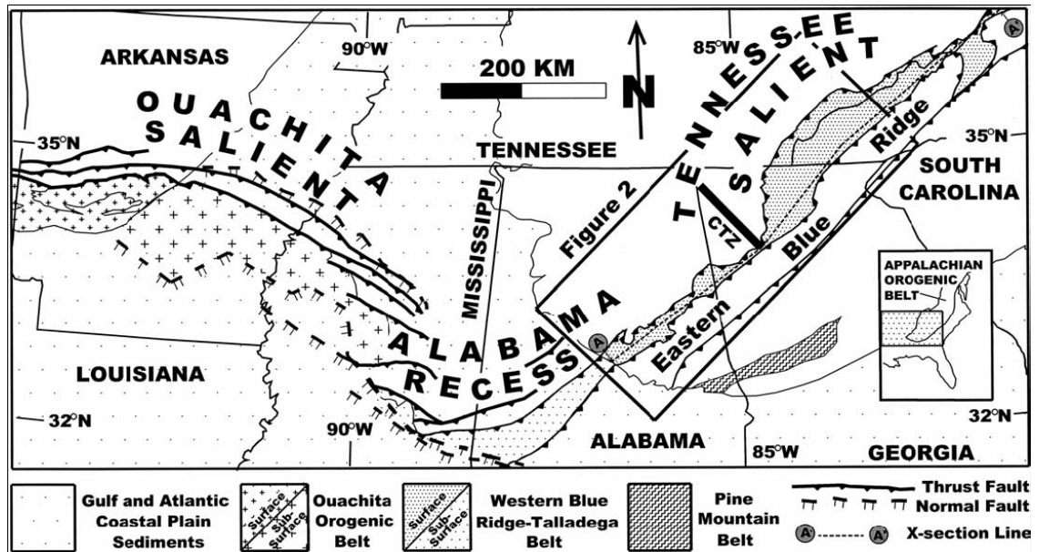
Figure 2-7. Regional map of the southwestern Appalachian orogen and the eastern Ouachita orogen, marking the location of a proposed transverse zone (labeled as CTZ) in northwestern Georgia, from Tull and Holm (2005). Also shown here is the location of cross section A–A' from Figure 2-8.
