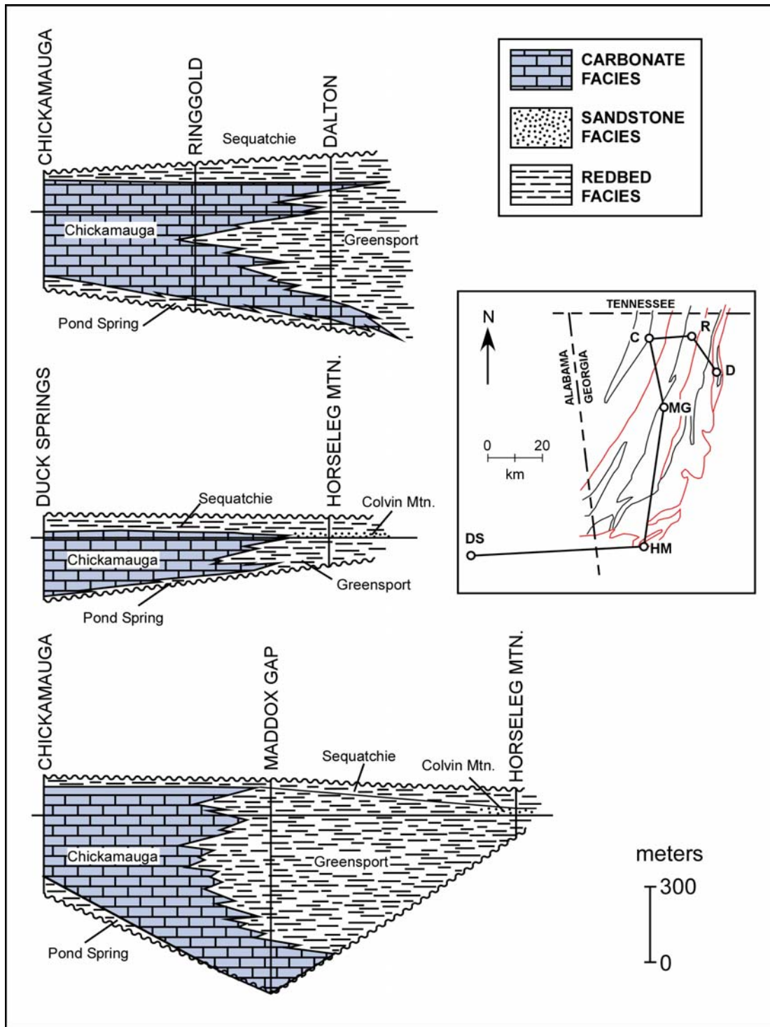
Figure 3-5. Cross sections of the Middle and Upper Ordovician showing the two dominant facies, modified from Carter and Chowns (1993) with field observations (thickness and correlation) for Maddox Gap. Generally, shallow-water carbonates of the Middle Ordovician Chickamauga Limestone predominate in the northwest and grade southeastward into peritidal clastic red bed facies of the Middle and Upper Ordovician Greensport and Sequatchie Formations.
