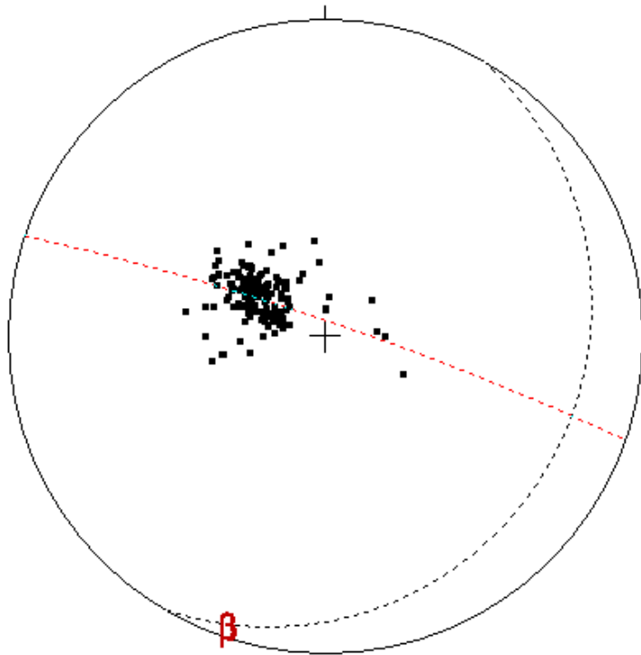
Figure 4-3 Equal-area stereonet plot of poles to bedding on Taylor Ridge monocline without small-scale fold
