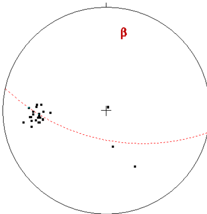
Figure 4-8 Equal-area stereonet of poles to bedding on Horn Mountain anticline
