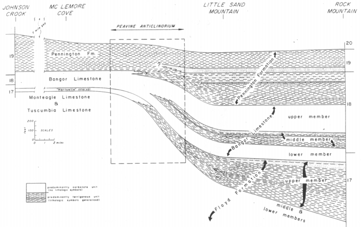
Figure 3-8. Alternate interpretations of the Mississippian succession in northwestern Georgia, from Rich (1986b).
