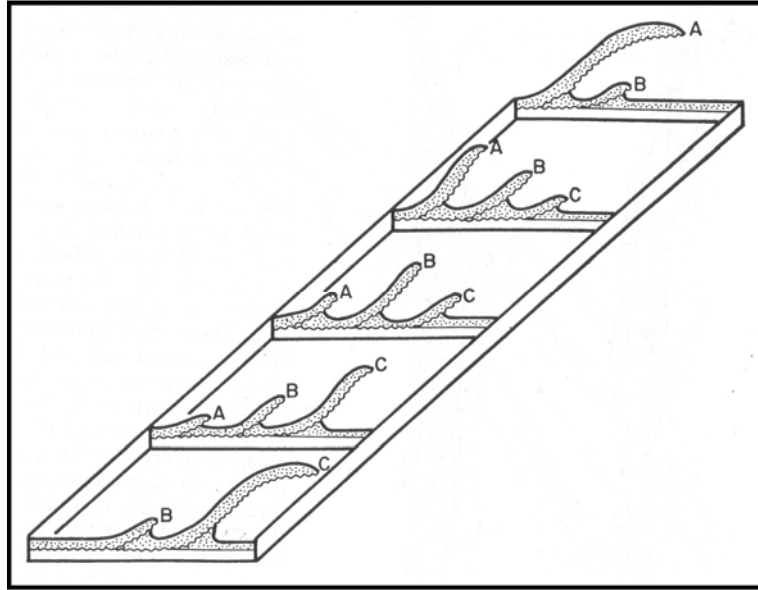
Figure 2-6. Diagram of the transfer of displacement within a thrust fault system, from Dahlstrom (1969).
