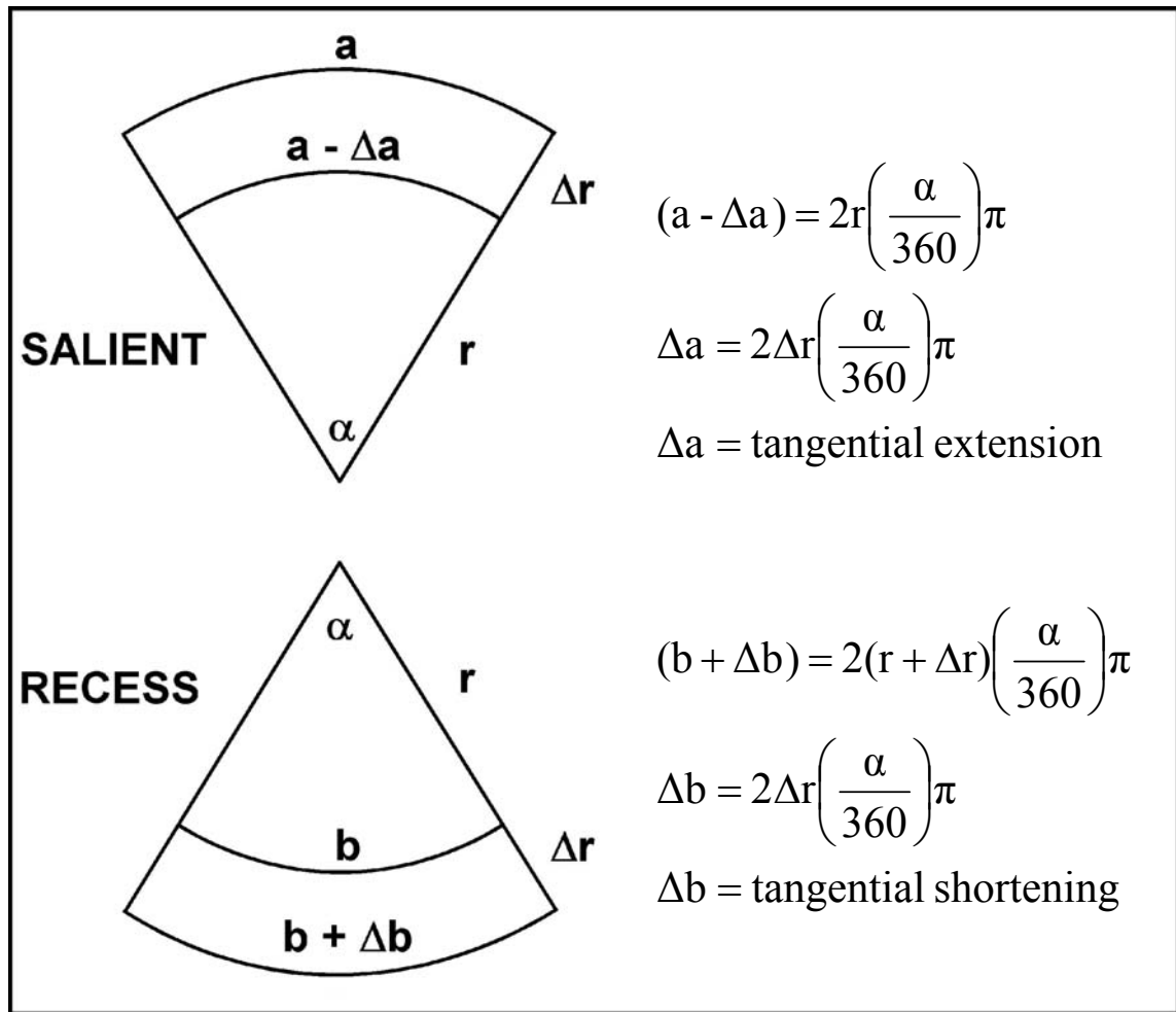
Figure 2-2. Sample calculations of implied tangential strain around a salient and a recess, adapted from Thomas (1989). Note that the sense of extension/shortening is reversed for palinspastic reconstructions.
