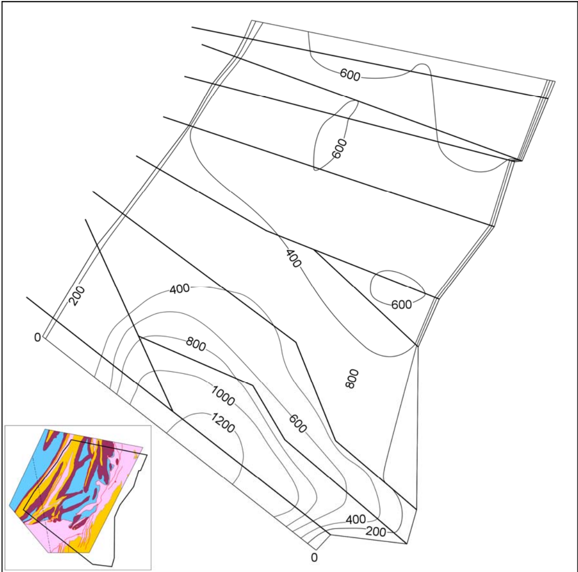
Figure 5-5. Isopach map of the restored-state ductile duplex using a simple line-length balance method for the base of the Knox Group (Unit 2). Location of area is shown on inset map. Cross sections used for data are shown as black lines. Contour values are in meters.
