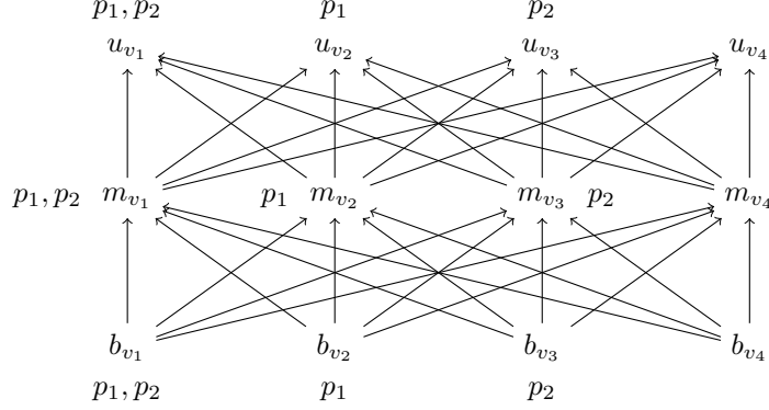
Fig. 1. The canonical asymptotic Kripke model M_{GL}^{\Phi} = (W, R, V) for \Phi = \{p_1, p_2\} , defined in Definition 3.1. The accessibility relation is the transitive closure of the one drawn in the picture. The figure shows only propositional atoms true at each world.
