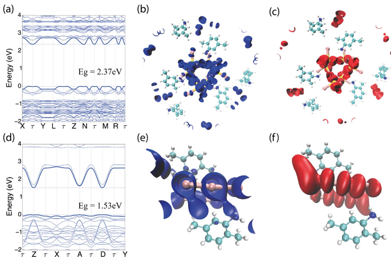
Fig. 4. DFT band structure calculations and charge densities at the bottom of the conduction band and the top of the valence band for 2,5-DMASnI 3 (a, b and c) and 2,5-DMAI 3 (d, e and f).
