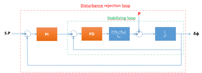
Figure 2: Cascade control.
