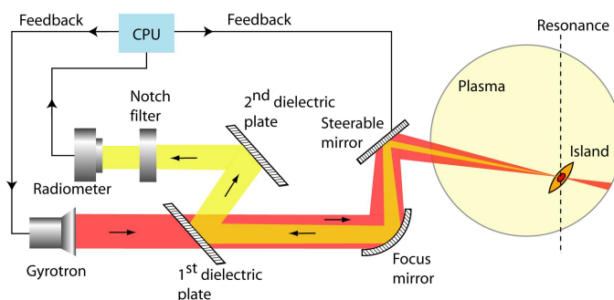
Fig. 2: Schematic overview of the in-line electron cyclotron emission - electron cyclotron resonance heating control system. The yellow beam gives the measurement signal of a few nanowatts, whereas the red beam is the microwave heating of one megawatt. The 'Notch filter' blocks the stray radiation such that both the actuation and the measurement can be performed using the same path. In other words, microwave radiation is deposited at the same location as it is being measured.
