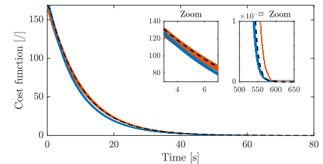
Figure 2: Simulation of (3) (—), Simulation of [3] (—), Lie bracket system (1) (—); \rho = 0.025 \text{ rad/s} , \omega_L = 2 \text{ rad/s}
