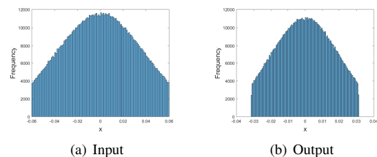
Figure 2: Beam Distributions
