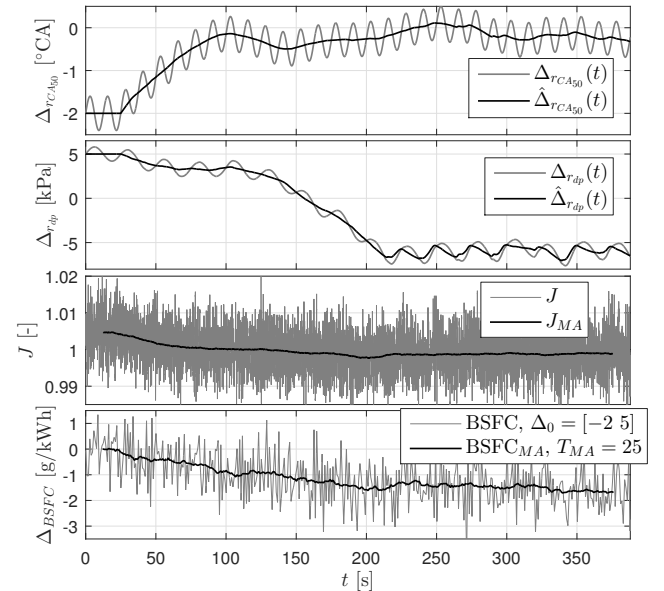
Figure 3: ES inputs \Delta r_{CA50} , \Delta r_{dp} , cost J and BSFC saving \Delta \text{BSFC} , and their moving averages J_{MA} , \Delta \text{BSFC}_{MA} .
