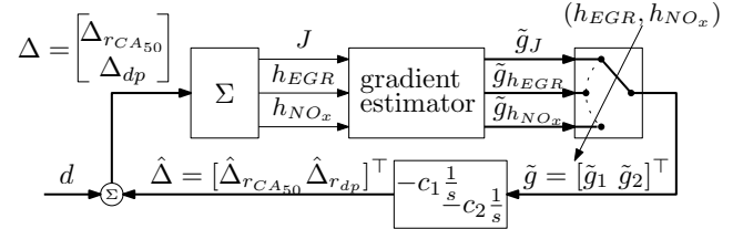
Figure 2: Extremum-seeking (ES) schematics. Signals in \mathbb{R}^{2 \times 1} indicated by thick arrows, scalar signals by thin arrows. c_1, c_2 > 0 are gradient descent optimizer gains.
