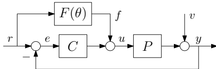
Figure 1: Control configuration for data-driven feedforward: the parameters \theta are iteratively optimized based on measured data.
