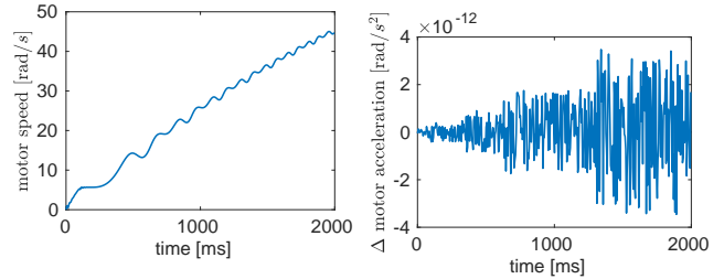
Figure 2: SimScape simulation
