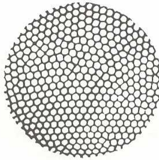
Figure 3.5: (Rayleigh-B enard convection) One of B enard’s original photographs, low resolution, seen from the top [107].
