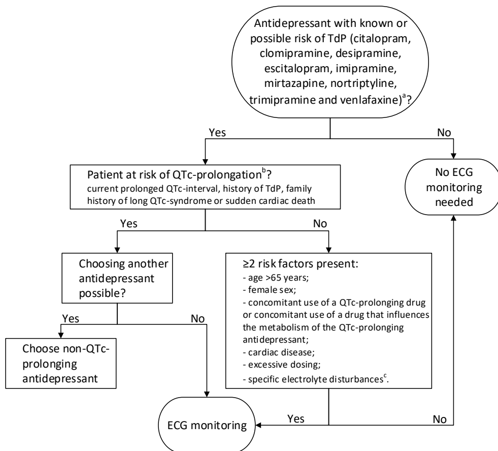
Figure 1. Decision tree for ECG monitoring with antidepressant treatment. a Based on CredibleMeds.org 5 , which represents available and evolving evidence that is constantly re-evaluated when new evidence becomes available; b If the risk of QTc-prolongation cannot be determined, it can be considered absent for decision making purposes; c In case of a strong suspicion of electrolyte disturbances, e.g. with alcoholism, anorexia nervosa, diarrhoea, use of loop diuretics, etc., the calcium, potassium and magnesium serum level should be quantified. QTc QT-interval corrected for heart rate; ECG electrocardiogram; TdP Torsade de Pointes.
