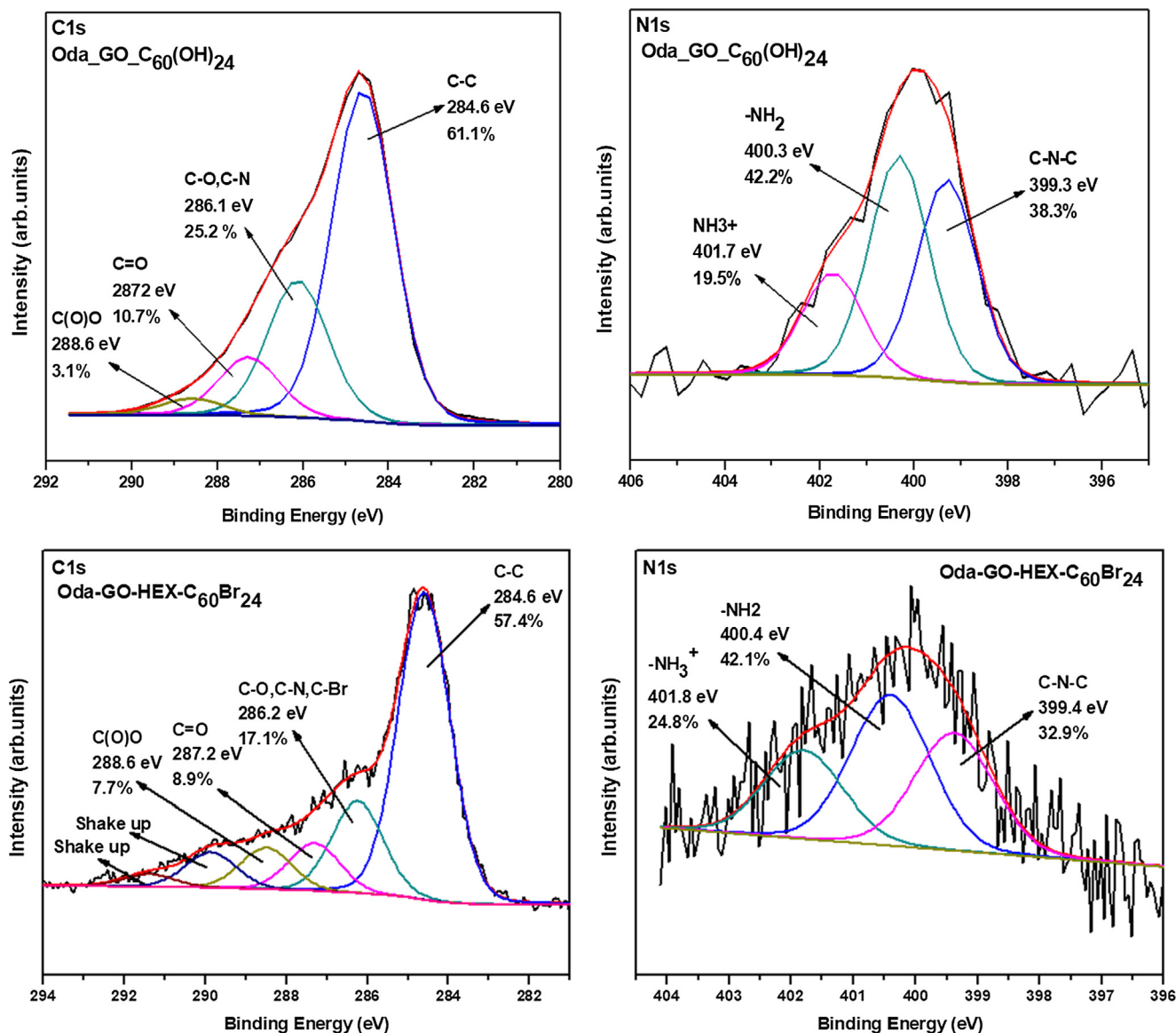
Fig. 7. Top: C1s (left) and N1s (right) core level X-ray photoemission spectrum of a ODA-GO- C_{60}(OH)_{24} hybrid multilayer film. Bottom: C1s (left) and N1s (right) core level X-ray photoemission spectrum of the ODA-GO-HEX- C_{60}Br_{24} hybrid multilayer film.
