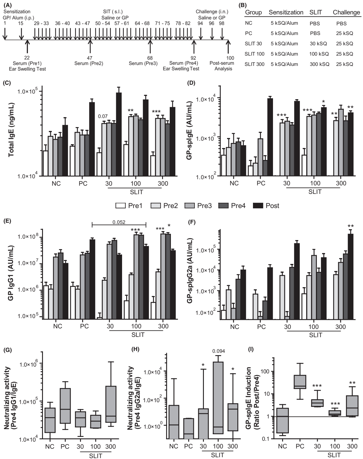
FIGURE 4 Overview and immunoglobulin response after GP-SLIT treatment. A, Outline of the SLIT protocol. B, Outline of the treatment groups. C, Serum levels of total IgE (ng/mL) taken before SLIT (white bars, Pre1), after 3 weeks of SLIT (light grey bars, Pre2), after 6 weeks of SLIT (middle grey bars, Pre3), before challenge (dark grey bars, Pre4), and after challenges (black bars, Post). D, Serum GP-splgE (Arbitrary Units (AU)/mL, Pre1-4, and Post). E, Serum GP-splgG1 (AU/mL, Pre1-4, and Post). F, Serum GP-splgG2a (AU/mL, Pre1-4, and Post). G, Neutralizing activity plotted as ratio of GP-splgG1/GP-splgE levels in Pre4-sera. H, Neutralizing activity plotted as ratio of GP-splgG2a/GP-splgE levels in Pre4-sera. I, Fold induction of GP-splgE after challenge (Post-sera/Pre4-sera). In Figure 4C-F, values are expressed as mean \pm SEM ( n = 8 ). In Figure 4G-I, values are expressed in box-and-whiskers plots (min-max). * P < .05 , ** P < .01 , and *** P < .005 compared to positive control at the same time-point. NC: negative control, PBS challenged; PC: positive control, GP challenged; 30, 100, 300: different doses of SCIT-treated mice (kSQ), GP challenged
