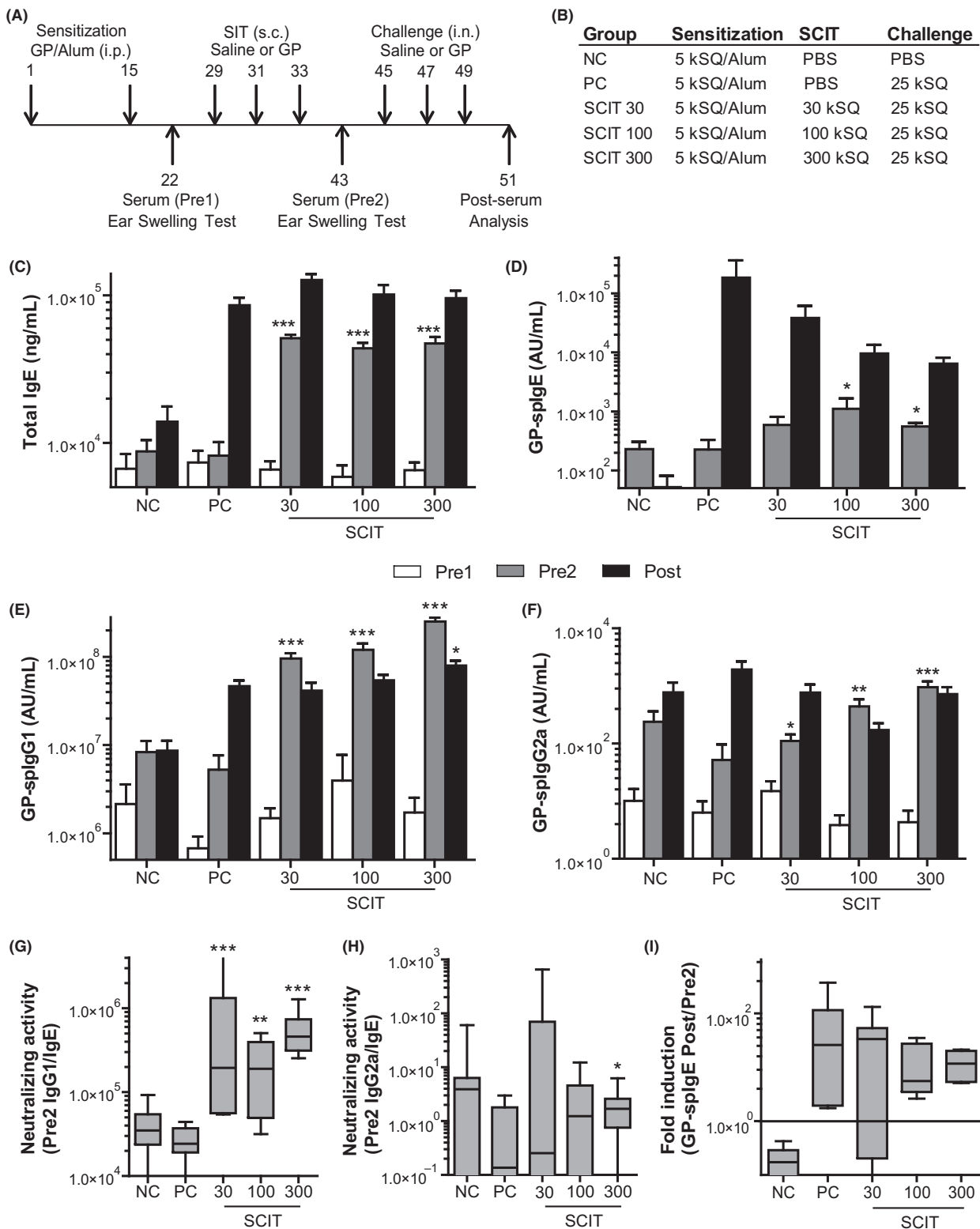
FIGURE 1 Overview and immunoglobulin response after GP-SCIT treatment. A, Outline of the SCIT protocol. B, Outline of the treatment groups. C, Serum total IgE (ng/mL) taken before SCIT (white bars, Pre1), before challenge (grey bars, Pre2), and after challenges (black bars, Post). D, Serum GP-splgE (Arbitrary Units (AU)/mL, Pre2, and Post). E, Serum GP-splgG1 (AU/mL, Pre1-2, and Post). F, Serum GP-splgG2a (AU/mL, Pre1-2, and Post). G, Neutralizing activity plotted as ratio of GP-splgG1/GP-splgE levels in Pre2-sera. H, Neutralizing activity plotted as ratio of GP-splgG2a/GP-splgE levels in Pre2-sera. I, Fold induction of GP-splgE after challenge (Post-sera/Pre2-sera). In Figure 1C-F, values are expressed as mean \pm SEM (n = 8). In Figure 1G-I, values are expressed in box-and-whiskers plots (min-max). * P < .05 , ** P < .01 , and *** P < .005 compared to PC at the same time-point. NC: negative control, PBS challenged; PC: positive control, GP challenged; 30, 100, 300: different doses of SCIT-treated mice (kSQ), GP challenged
