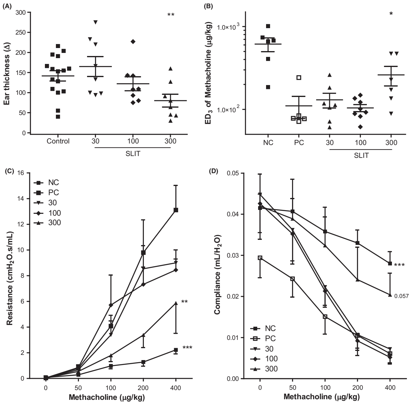
FIGURE 5 Clinical manifestations after GP-SLIT treatment. A, IgE-dependent allergic response plotted as net ear thickness ( \mu\text{m} ) 2 hours after GP injection (1kSQ) in the right ear and PBS in the left ear as a control, performed after SLIT. Placebo-SLIT-treated mice were plotted together as Controls (NC and PC). B, Effective dose (ED) of methacholine, when the airway resistance reaches 3 \text{cmH}_2\text{O.s/mL} (ED 3 ). C: Airway hyperreactivity (AHR) was measured by FlexiVent and plotted as airway resistance (R in \text{cmH}_2\text{O.s/mL} ) and as D: airway compliance (C in \text{mL/cmH}_2\text{O} ). Absolute values are expressed as mean \pm SEM ( n = 8 ). * P < .05 , ** P < .01 , and *** P < .005 compared to PC. NC: negative control, PBS challenged; PC: positive control, GP challenged; 30, 100, 300: different doses of SLIT-treated mice (kSQ), GP challenged
