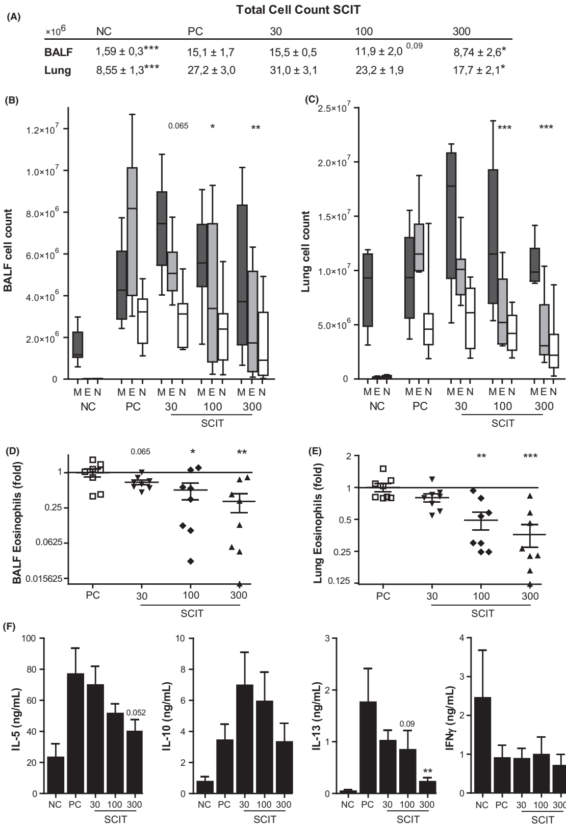
FIGURE 3 The eosinophilic and cytokine response after GP-SCIT treatment. A, Total cell counts in bronchoalveolar fluid (BALF) and lung single cell suspensions (Lung). B, Differential cytopsin cell counts in BALF and in C, lung. M, mononuclear cells; E, eosinophils; N, neutrophils. Absolute numbers are plotted in box-and-whiskers plots (min-max). D, BALF eosinophils and E, lung eosinophils, both plotted as ratio of suppression (absolute eosinophils/average PC eosinophils; mean \pm SEM). F: Net levels of IL-5, IL-10, IL-13, and IFN \gamma measured in restimulated lung single cell suspensions. Concentrations were calculated as the concentration after restimulation minus control (mean \pm SEM, n = 8). * P < .05, ** P < .01, and *** P < .005 compared to PC. NC: negative control, PBS challenged; PC: positive control, GP challenged; 30, 100, 300: different doses of SCIT (kSQ), GP challenged
