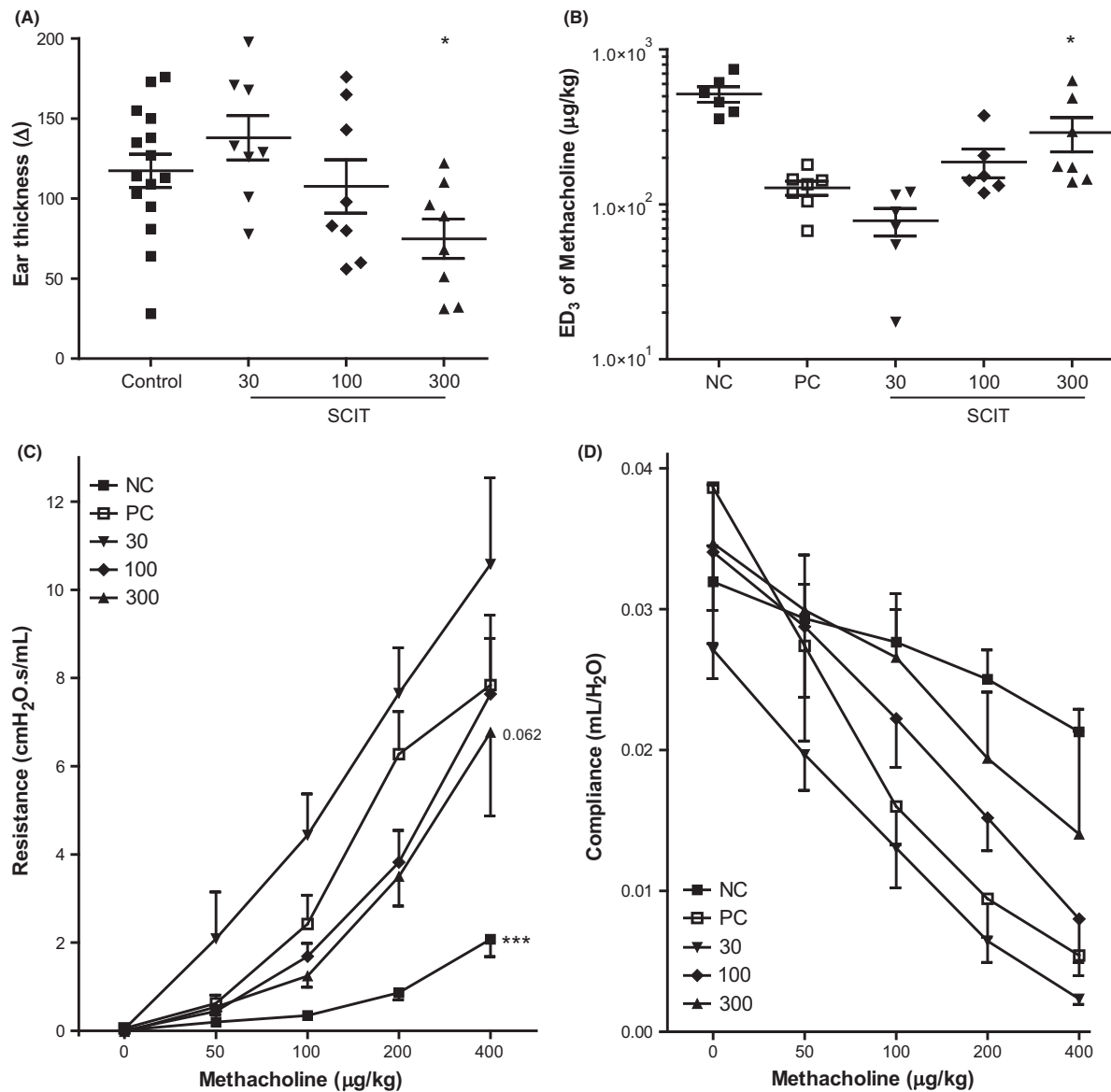
FIGURE 2 Clinical manifestations after GP-SCIT treatment. A, IgE-dependent allergic response plotted as net ear thickness ( \mu\text{m} ) two hours after GP injection (1kSQ) in the right ear and PBS in the left ear as a control, performed after SCIT. Placebo-SCIT-treated mice were plotted together as Controls (NC and PC). B, Effective dose (ED) of methacholine, when the airway resistance reaches 3 \text{ cmH}_2\text{O.s}/\text{mL} (ED 3 ). C, Airway hyperreactivity (AHR) was measured by FlexiVent and plotted as airway resistance (R in \text{cmH}_2\text{O.s}/\text{mL} ) and as D, airway compliance (C in \text{mL}/\text{cmH}_2\text{O} ). Absolute values are expressed as mean \pm SEM ( n = 8 ). * P < .05 , ** P < .01 , and *** P < .005 compared to PC. NC, negative control, PBS challenged; PC, positive control, GP challenged; 30, 100, 300: different doses of SCIT (kSQ), GP challenged
