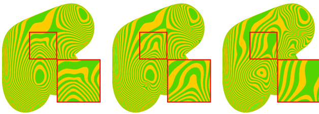
Figure 7: A comparison of \mathbf{n}_L (left), \mathcal{A}_3 (mid) and \mathcal{A}_4 (right) for a Loop subdivision surface.
