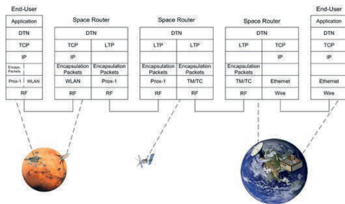
Fig. 6. Communication scenario – protocol stack [13].
