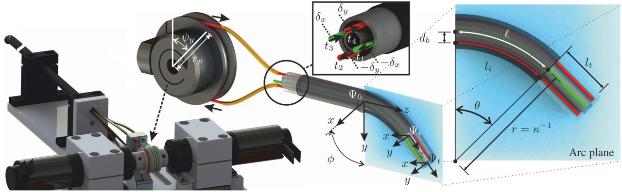
Fig. 2. An overview of the robotically actuated delivery sheath (RADS). The articulating tip of the RADS is actuated in two degrees of freedom by two pairs (red and green) of antagonistic-configured tension wires driven by two pulleys with radii ( r_p ) and angles ( \psi_x and \psi_y ). Three coordinate systems are assigned to describe the tip pose of the RADS: \Psi_0 is the reference frame fixed to the shaft, \Psi_i is the intermediate frame assigned to the arc section and frame ( \Psi_t ) is fixed to the articulating tip. Displacement of the tension wires ( t_1, \dots, t_4 ) by \delta_x and \delta_y (inset centre) results in instrument bending along the x - and y -axes (frame ( \Psi_0 )), respectively. The arc of the RADS with parameters, bend angle ( \theta ), backbone length ( \ell ), radius ( r ) and curvature ( \kappa ) lies in a plane described by the arc plane (inset right). The orientation of the arc plane about the z -axis of the reference frame ( \Psi_0 ) is denoted by angle ( \phi ). Further, the tendon distance to the backbone arc ( \ell ) is denoted d_b . A rigid link (not completely shown) of length ( l_t ) is attached to the arc (frame ( \Psi_i )) of the RADS.
