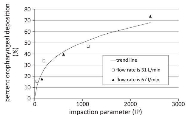
Fig. 2. Percent oropharyngeal deposition as a function of the impaction parameter ( IP = \rho \cdot D^2 \cdot \Phi ). Data points derived from the Usmani study [24].
