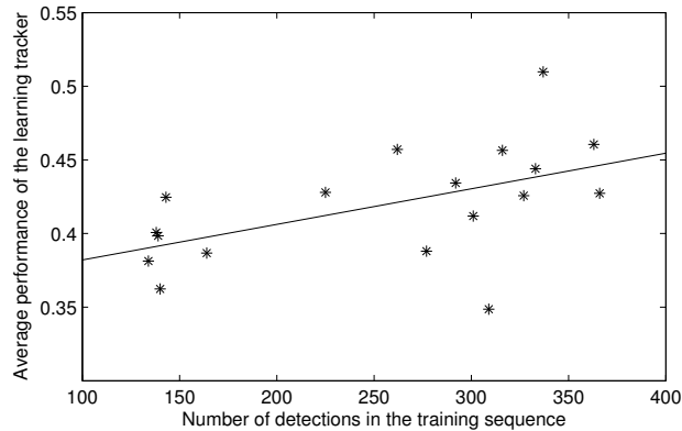
Figure 3: Learning tracker performance score depends on the amount of training data. Performance score measures overlap between detection and tracker estimate, as explained in section 3.3. The line shows the best least-squares fit of a first-order polynomial to the data.
