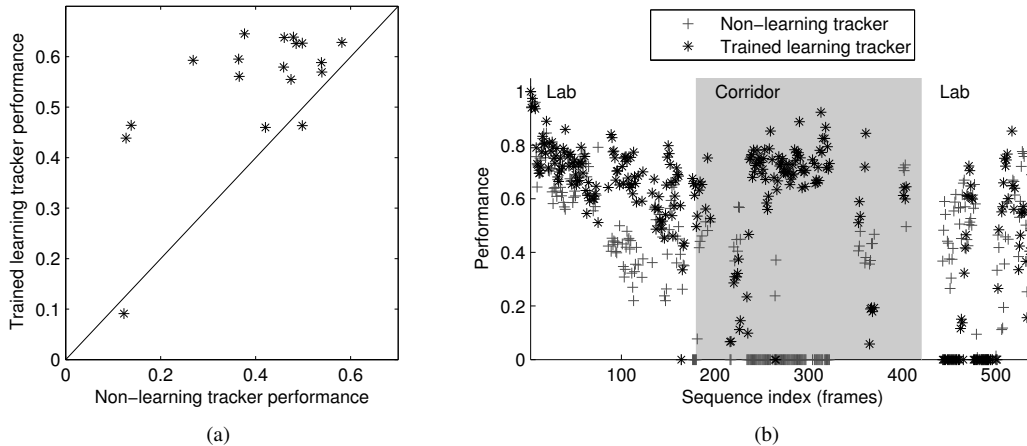
Figure 2: (a) Performance on all test sequences for the learning tracker and the non-learning tracker. Points above the x = y line have a higher performance for the learning tracker. (b) Performance of both tracker types over time evaluated on one test sequence. The non-learning tracker suffers as conditions change. Performance is a measure of overlap between detection and tracker estimate, as explained in section 3.3.
