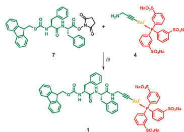
Scheme 1 Synthesis of the Fmoc-protected, dipeptidic Au(I)-metalloamphiphile 1 : (i) DMF, rt; 29% yield after purification with size-exclusion chromatography.
