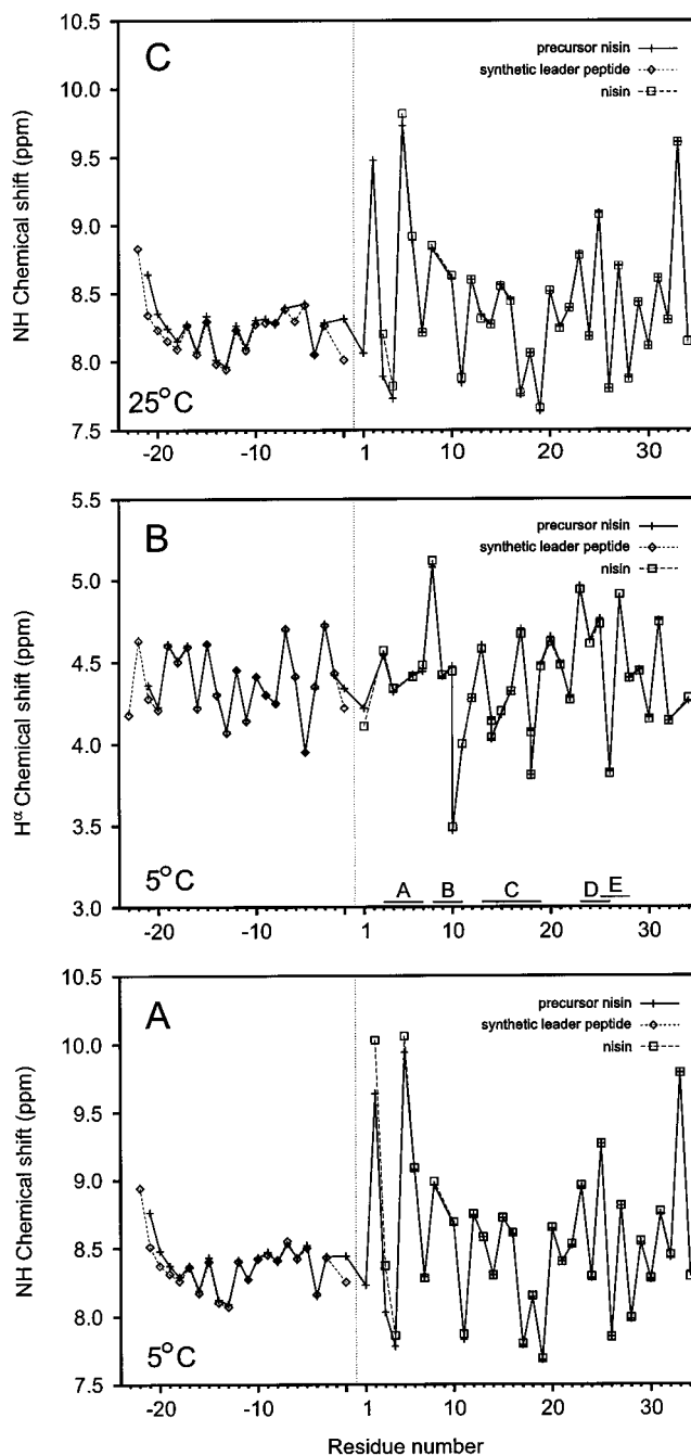
FIGURE 3: Chemical shifts (in ppm) of backbone protons of precursor nisin (+, solid line), of the synthetic leader peptide (<math>\diamond</math>, dotted line), and of nisin (□, dashed line) versus the residue number. Chemical shifts were obtained from NMR spectra of all three molecules in an aqueous solution of pH 3.5. (A) Chemical shifts of NH protons derived from NMR spectra recorded at 5 °C, (B) chemical shifts of H α protons from measurements at 5 °C, and (C) chemical shifts of NH protons at 25 °C. The positions of the lanthionine rings A–E in nisin and in precursor nisin are indicated in (B).
