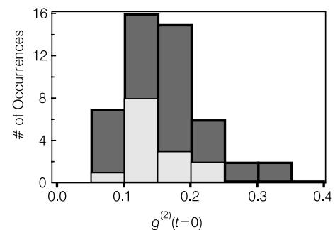
FIG. 4. Histogram of the g^{(2)}(0) values obtained from the time traces of 50 bichromophores before the first intensity drop (dark bars). For comparison, the histogram of 14 single PM chromophores is also shown (light bars).
