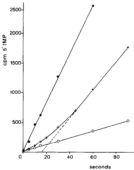
FIG. 3. Transient kinetics of the hydrolysis of [ ^3\text{H} ]cIMP by the cGMP-dependent phosphodiesterase isolated from the cellular slime mold D. discoideum (5). The enzyme was rapidly mixed with 0.1 \mu\text{M} [ ^3\text{H} ]cIMP (containing about 20,000 cpm). The reactions were terminated at the times indicated, and the reaction mixture was chromatographed on 0.3-ml reverse-phase columns. ○, [ ^3\text{H} ]5'-IMP formed after mixing nonactivated enzyme with [ ^3\text{H} ]cIMP. ●, The enzyme was preincubated with 0.5 \mu\text{M} \text{c}^8\text{b-GMP} for 5 min; at t = 0 the activated enzyme was mixed with [ ^3\text{H} ]cIMP and 0.5 \mu\text{M} \text{c}^8\text{b-GMP} . +, The enzyme was not preactivated by \text{c}^8\text{b-GMP} ; however, activation was started at t = 0 by mixing the nonactivated enzyme with [ ^3\text{H} ]cIMP and 0.1 \mu\text{M} \text{c}^8\text{b-GMP} .
