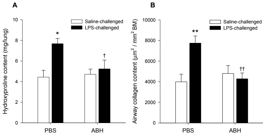
Figure 5: Whole lung hydroxyproline content (A) and collagen content in the airway wall (Sirius red; B) in guinea pigs challenged repeatedly with LPS or saline and treated with inhaled ABH or PBS (control). Data represent means \pm SEM of 5-8 experiments. Hydroxyproline determinations were performed in triplicate and 2 to 6 airways were analysed for each animal for the Sirius red staining. * P < 0.05 , ** P < 0.01 vs saline-challenged control; † P < 0.05 , †† P < 0.01 vs LPS-challenged control.
