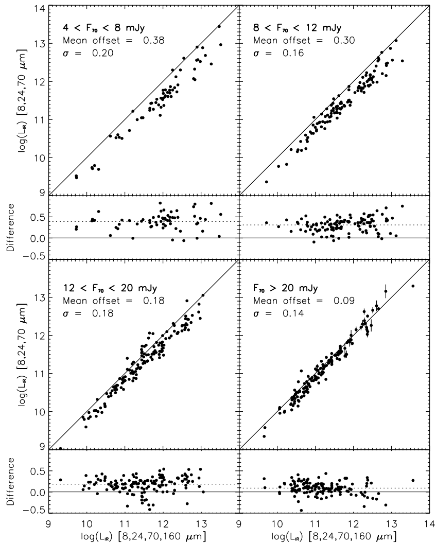
Figure 14. Same as Figure 13 but divided into four 70 \mu\text{m} flux bins. Note that the mean offset between the two luminosity estimates decreases at higher 70 \mu\text{m} fluxes, while the overall scatter stays about the same.
