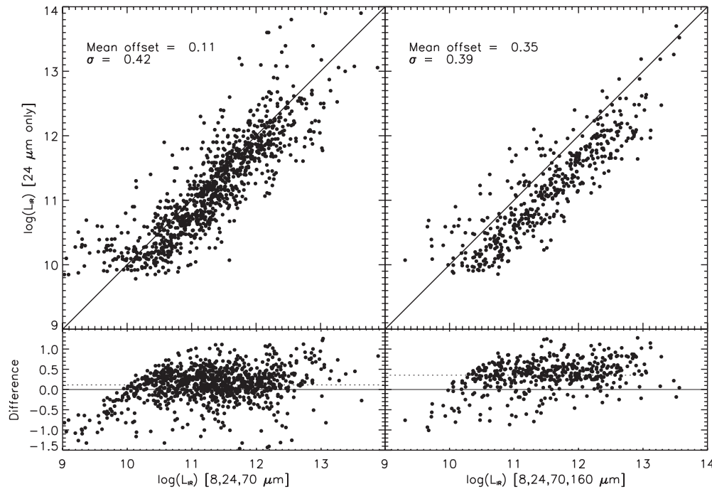
Figure 20. Comparison of luminosities obtained with all the available bands for the sources without 160\ \mu\text{m} detections (left) and those with 160\ \mu\text{m} detections (right) to the luminosities obtained from just the 24\ \mu\text{m} data point. The dotted line represents the mean difference between the two and the \sigma value is the internal dispersion about that mean. The sources detected at 160\ \mu\text{m} show a similar offset in their luminosities as they did in the 70/160\ \mu\text{m} luminosity comparison (see Figure 13). This is a further indication that the sources detected at 160\ \mu\text{m} are intrinsically different (i.e., have a colder dust component) than those that are not.
