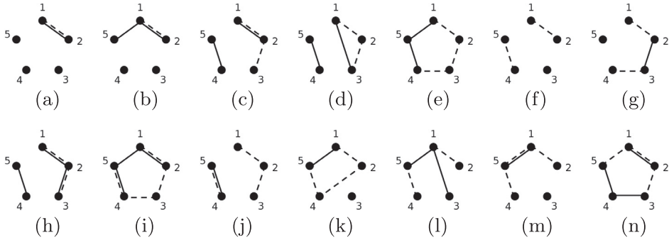
Fig. 1. Graphs fulfilling the conditions in Subsection 5.2, used to represent the support of the set of zeros of a matrix. A dashed edge between vertices i and j represents a zero with support \{i, j\} , whilst a solid edge between the vertices i and j represents a zero with support \{1, \dots, 5\} \setminus \{i, j\} .
