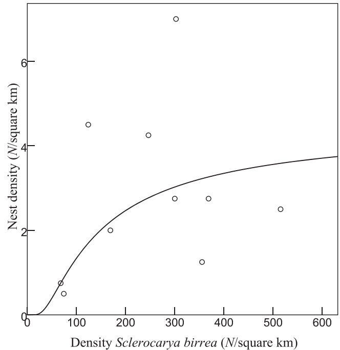
FIGURE 2. S-curve regression model for nest density and the number of Sclerocarya birrea trees \geq 8 m high inside nest census areas (compare Fig. 1).
