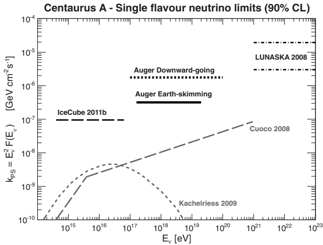
Figure 5. Upper limits at 90% CL on a single flavor E_{\nu}^{-2} flux from the active galaxy Centaurus A from the Earth-skimming and downward-going neutrino analyses, together with bounds from the IceCube Neutrino Observatory (Abbasi et al. 2011b) and LUNASKA (James et al. 2011). The predictions for two models of UHE \nu production—in the jets (Cuoco & Hannestad 2008), and close to the core of Centaurus A (Kachelriess et al. 2009)—are also shown.
