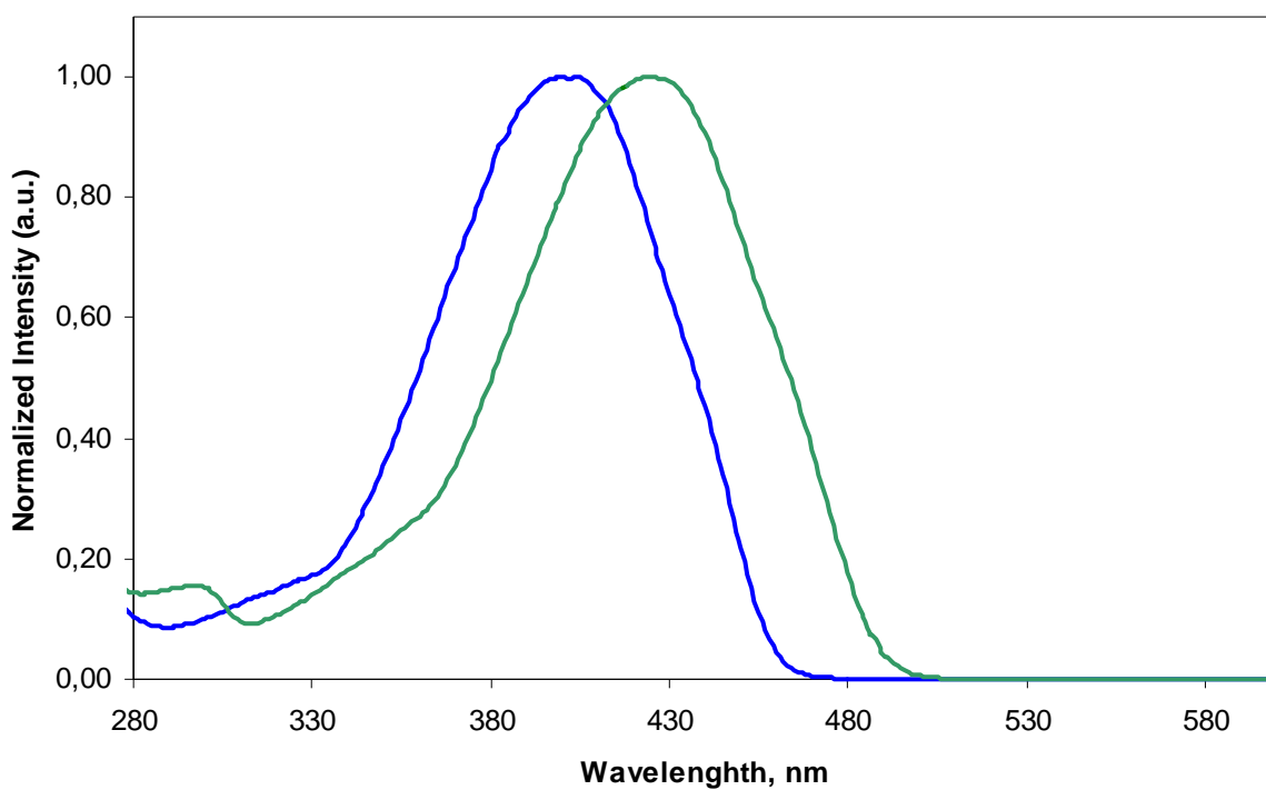
Figure S 3. UV-Vis absorbance spectra for monochlorosilyl-functionalized oligothiophenes 9 (blue curve) and 10 (green curve) in dilute THF solutions at 40 °C.
