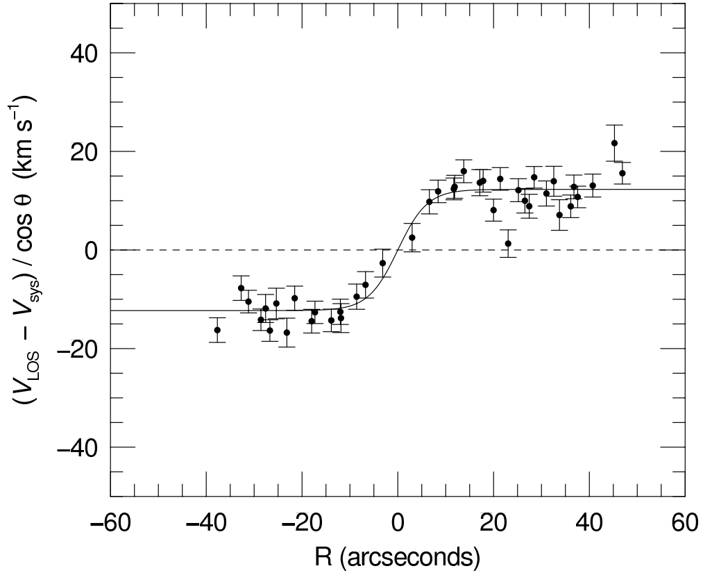
Fig. 16.— \text{H}\alpha projected rotation curve for UGC 6897 as an example of the very low-levels of projected rotation that can be detected using SparsePak and the echelle grating, and used to derive precise inclinations from iTF. Line-of-sight velocities ( V_{\text{LOS}} ) are extracted from \pm 30^\circ wedge about the determined kinematic major axis, corrected for systemic recession velocity ( V_{\text{sys}} ), and corrected for azimuthal projection (only). A model rotation curve with projected amplitude of 12.3 \pm 0.7 \text{ km s}^{-1} about the barycenter is shown as a solid line.
