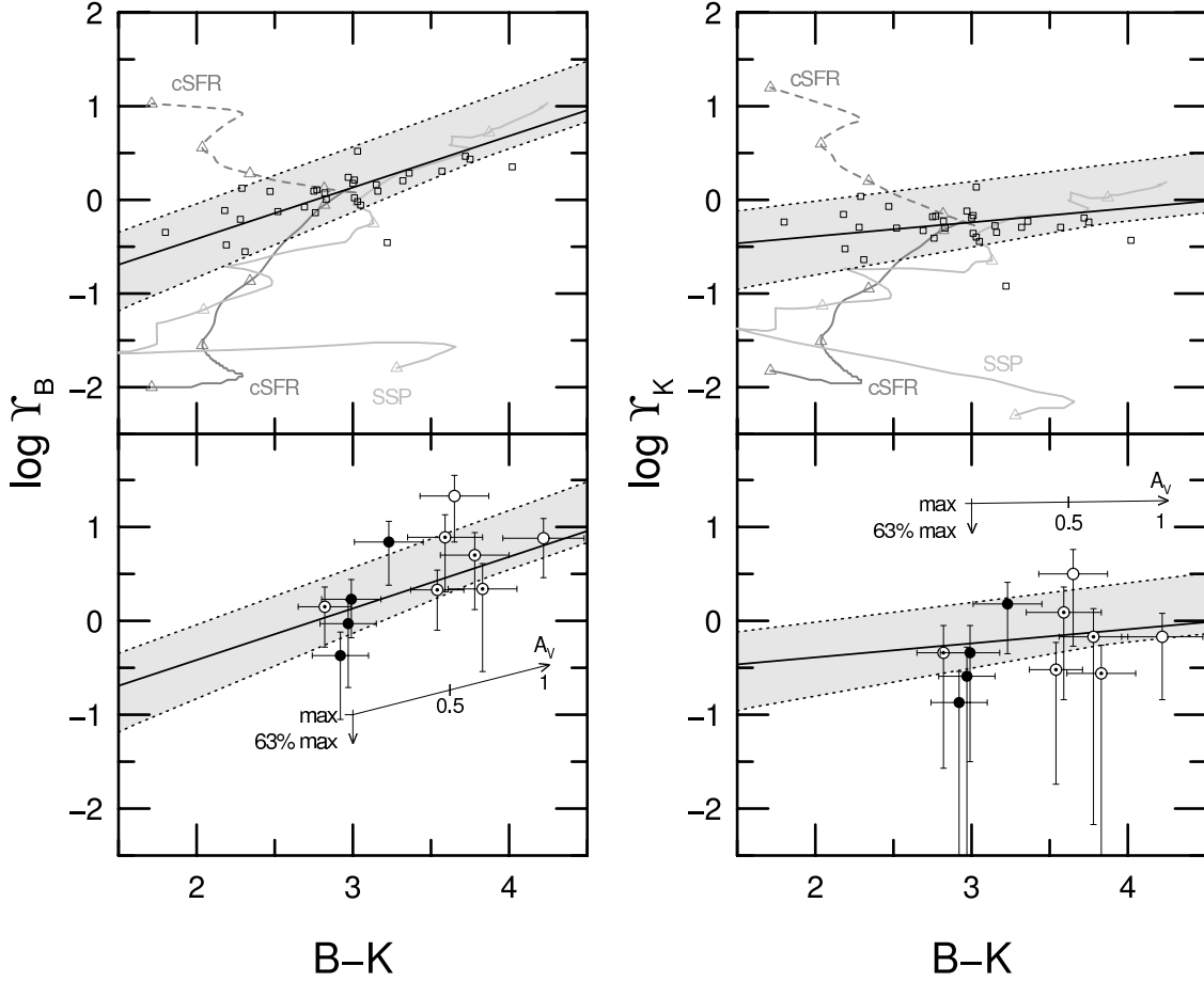
Fig. 2.— B - and K -band \Upsilon versus B - K color. Models : Solid black line and gray areas represent mean and extrema \Upsilon_* for the full range of SPS models given in Bell & de Jong (2001); they scale their IMF such that no galaxies in the Verheijen (1997) sample are super-maximal (see text). Trends in \Upsilon_* for SSP and cSFR models are plotted in the top panels as light and medium-gray lines punctuated by triangles marking age in time-steps from 10^7 to 10^{10} years in equal dex intervals (Bruzual & Charlot 2003). For cSFR, \Upsilon_{\text{dyn}}^{\text{disk}} is also calculated including gas mass in future star-formation up to 10^{10} years (dashed line). Observations : \Upsilon_{\text{dyn}}^{\text{disk}} values and uncertainties for galaxy disks in the literature (see text). Open squares are estimates (Sanders & Verheijen 1998; top panel) based on rotation-curve decomposition assuming MOND for the same sample of galaxies later used by Bell & de Jong (2001). Circles (bottom panel) represent the Bottenga (1993) sample, based on direct kinematic measurement marked here by inclination for face-on ( i < 30^\circ ; filled), highly-inclined ( 70^\circ < i < 80^\circ ; dotted), and edge-on ( i > 80^\circ ; open) systems. Reddening vectors are indicated, marked for 0.5 and 1 mag of visual extinction ( A_V ) in a foreground screen. Change in \Upsilon_* from a so-called maximum disk (providing up to 85-90% of the observed galaxy rotation) to a disk which provides only 63% of this rotation is also indicated.
