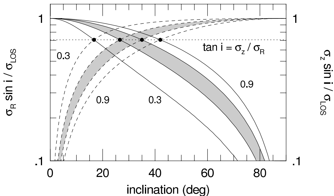
Fig. 6.— Projection of vertical and radial disk velocity-dispersion components ( \sigma_z , solid lines; \sigma_R , dashed line) into the minor-axis line-of-sight as a function of inclination. Curves represent different assumed SVE shape parameterized by the ratio \sigma_z/\sigma_R . Ratios of 0.5 to 0.7, expected to be typical for galaxies in our survey (Paper II), are high-lighted in grey. Horizontal, dotted-line intersections with curves mark inclinations where radial and vertical projections are equal. Inclination values ( i ) at these intersections are related to the SVE axis ratio, as given in the figure.
