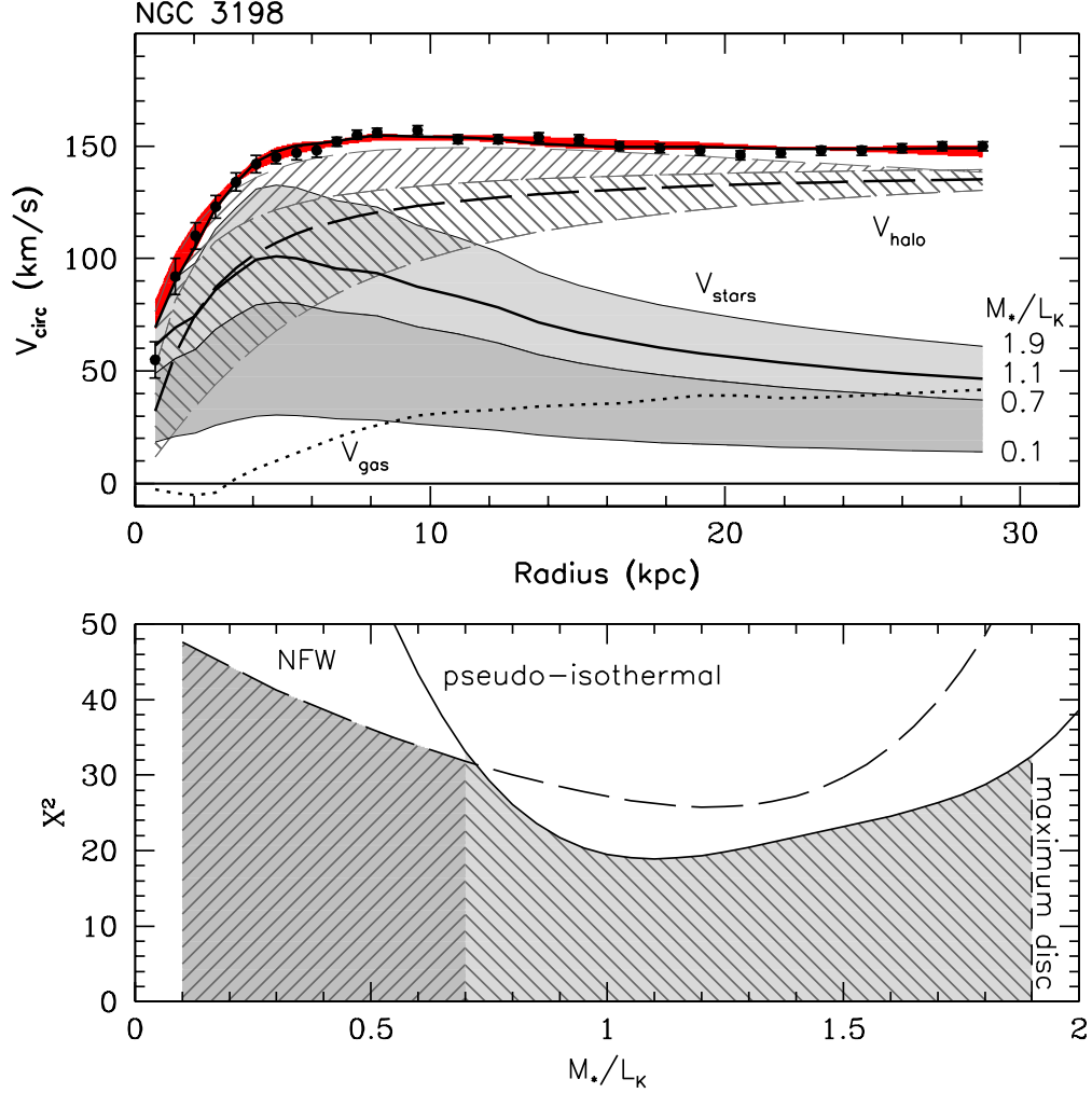
Fig. 1.— Example mass-decompositions for NGC 3198 for a factor of \sim 20 range in K -band \Upsilon_* (assumed constant with radius), constrained by the observed 21 cm (H I) rotation curve (points) and gas mass surface-density, adopting either a spherical pseudo-isothermal or NFW dark-matter halo profile. Stellar and halo mass-ranges (upper panel) are grey-scale coded (medium and light) for the break-point between halo models seen in the formal \chi^2 in the bottom panel. Total mass for the full range of \Upsilon_* is shown (upper panel) in red (dark grey). All \Upsilon_* values provide indistinguishably good fits to the observed rotation curve given the amplitude of non-axisymmetric motion (see text). The disk radial scale-length is 2.7 kpc. [COLOR IN ELECTRONIC EDITION ONLY]
