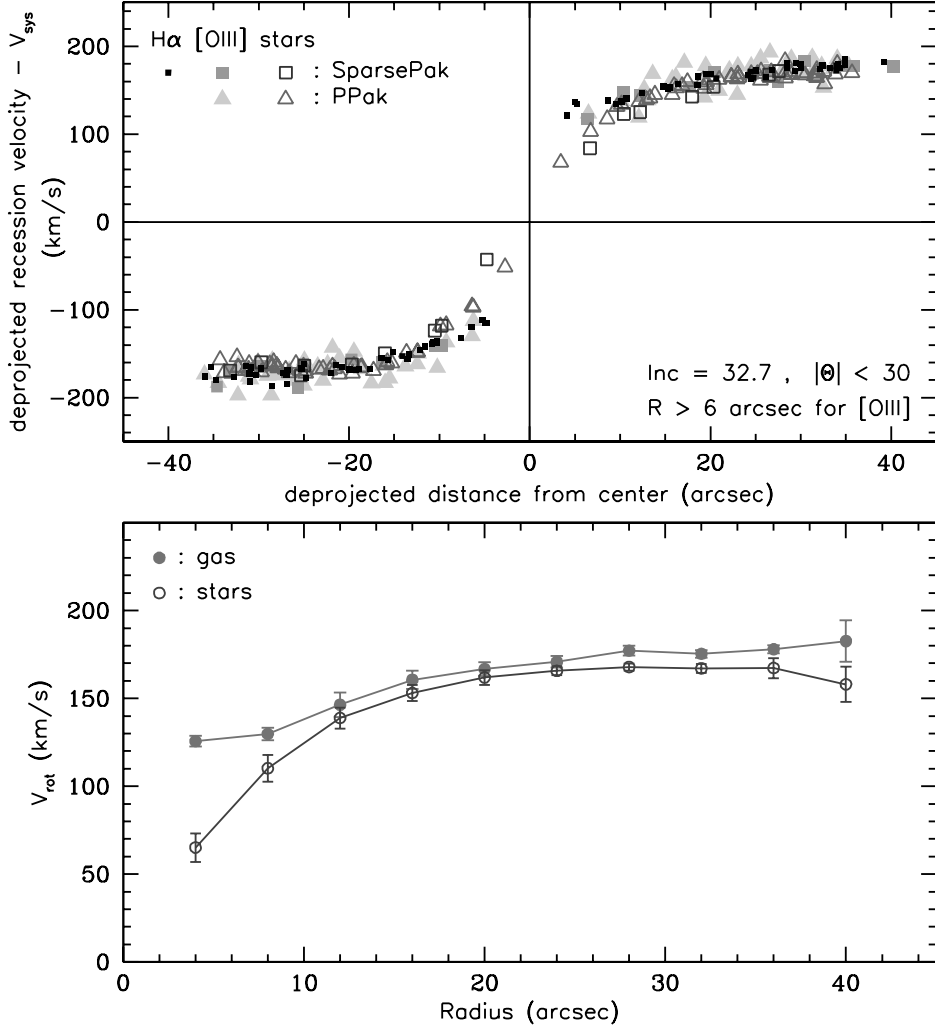
Fig. 17.— Asymmetric drift between the de-projected tangential velocities of stars (open squares and triangles) and ionized gas (filled grey squares and triangles for [\text{O III}]\lambda 5007 ; small, filled squares for \text{H}\alpha ) in UGC 6918, as observed with SparsePak and PPak. Gas velocities are based on line centroids, while stellar velocities are from cross-correlation with stellar templates in the same ( \text{Mg Ib} ) spectral region. The top panel shows deprojected tangential velocities for individual fibers within 30^\circ of the kinematic major axis, adopting a kinematic inclination of 32.7^\circ , and corrected for the systemic recession velocity, V_{\text{sys}} . The bottom panel gives the amplitude of the deprojected tangential velocity for gas and stars, V_{\text{rot}} , derived from tilted ring fits to radial bins of fibers, adopting the same inclination for each bin, and combining all SparsePak and PPak data shown in the top panel.
