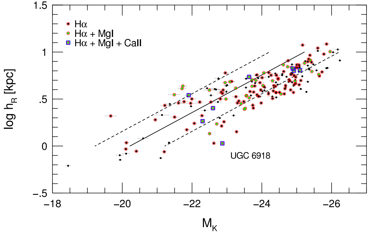
Fig. 14.— Size versus luminosity for the DMS, with sources marked as in Figure 10. Size corresponds to the disk scale-length, h_R , measured on red POSS images. Luminosity is measured in the K -band. Diagonal lines correspond to constant mean surface-brightness assuming disks dominate the integrated luminosity for Freeman surface-brightness disks of color B - K = 2.3, 3.3, and 4.3 (left to right, respectively). [COLOR]
