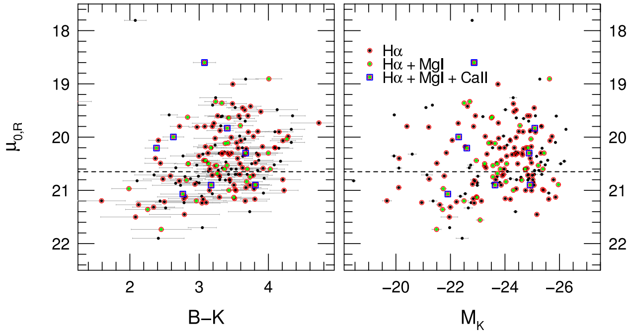
Fig. 13.— Distributions in B - K color, K -band absolute magnitude, M_K , and red disk central surface-brightness, \mu_{0,R} for the DMS, with sources marked as in Figure 10. The approximate Freeman surface-brightness is indicated by the horizontal dashed line. [COLOR]
