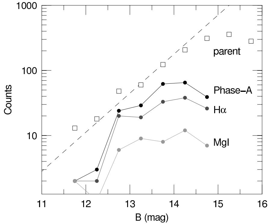
Fig. 11.— B -band galaxy counts (per 0.5 mag) for sub-samples in our survey selected from the UGC. The dashed line has a Euclidean slope of 0.6 dex, with an arbitrary normalization. The curved marked “ H\alpha ” represents the Phase-A sample with H\alpha IFS. The curve marked “MgI” is the subset of the Phase-B sample with Mg I IFS.
