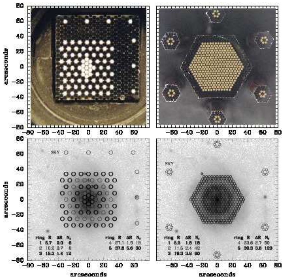
Fig. 3.— (Top row) Fiber integral-field units (IFU) developed for the DiskMass Survey, shown at the same angular scale: SparsePak (left, WIYN 3.5m telescope) and PPak (right, Calar Alto 3.5m telescope). Both IFUs subtend approximately 70 arcsec field in their core, sample with 4.7 and 2.7 arcsec diameter fibers, respectively, and reformat to feed grating-dispersed spectrographs in long-slit mode. Relevant spectrograph configurations, achieving 8000 < \lambda/\delta\lambda < 11000 are given in Table 1. (Bottom row) SparsePak and PPak overlays on UGC 6918 B -band image from the KPNO 2.1m telescope, with examples of azimuthal rings of fibers identified. Inset tables specify mean sky-plane radius ( r ), half-range of radius ( \Delta r ) for fiber centers, and number of fibers per ring ( N_f ).
