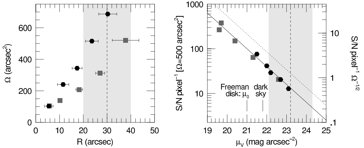
Fig. 4.— (Left panel) Solid-angle versus radius in five radial bins for SparsePak (grey squares) and PPak (black hexagons). Horizontal bars represent radial range in fiber centers for each bin. (Right panel) S/N per pixel as a function of V -band surface-brightness for stellar absorption-line spectroscopy in the Mg Ib region in a ring subtending 500 \text{ arcsec}^2 . Rightmost vertical scale gives equivalent S/N per \text{arcsec}^2 . Data for UGC 6918 (SparsePak) and UGC 1635 (PPak) are scaled to this \Omega and typical total integration-times with these instruments (12 and 8 hr, respectively). Diagonal lines are the predicted, detector-limited performance for the typical (solid) and longest (dotted) total integration times. In both panels grey shaded regions in both panels mark the distribution of apparent size and surface-brightness at 2.25h_R encompassing 90% of the galaxies in the DiskMass sample; vertical dashed lines represent median values.
