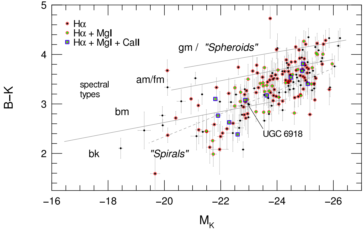
Fig. 12.— Optical–near-infrared color–absolute-magnitude diagram for the DMS, with sources marked as in Figure 10. Trends for spirals, spheroidals, and galaxies classified by spectral type from Bershady (1995) are marked with lines over the observed luminosity range in that survey, and labeled for reference (see text). The location of UGC 6918 is marked. [COLOR]
