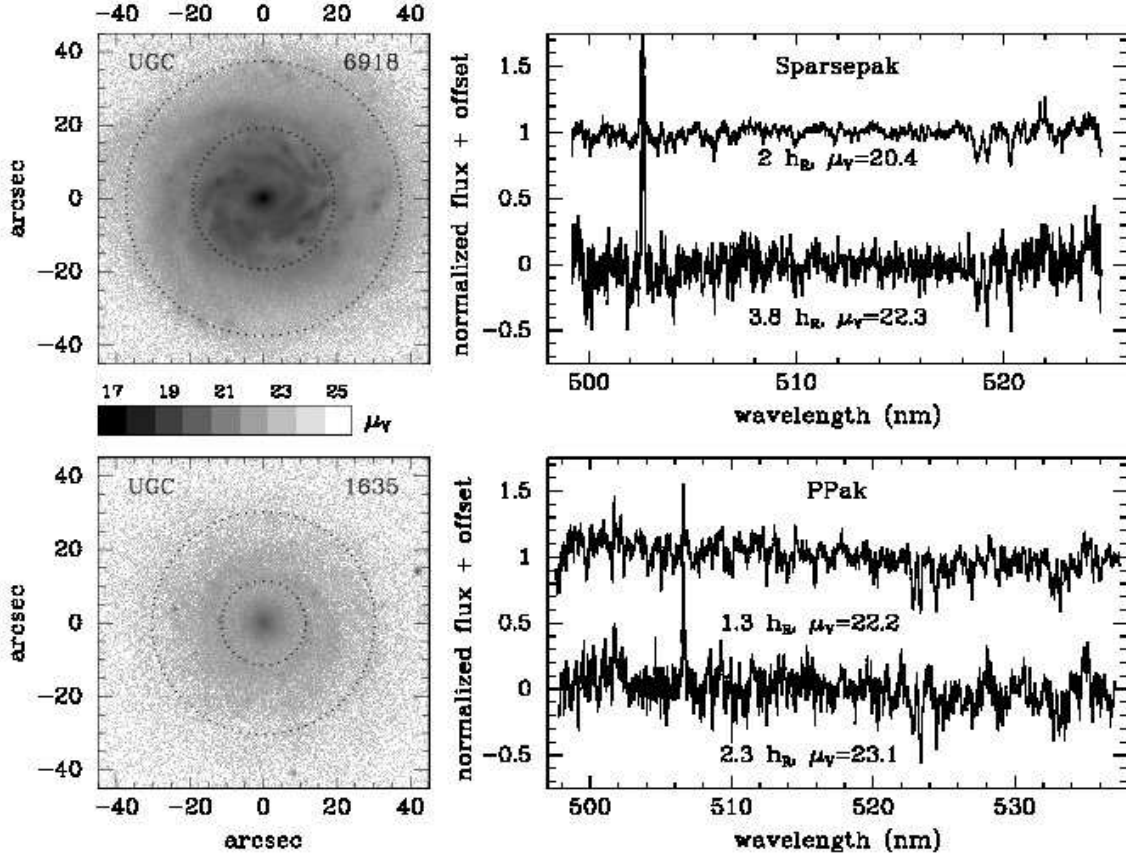
Fig. 5.— Survey spectroscopic dynamic range in surface-brightness, shown with KPNO 2.1m V -band images (60 sec exposures) and spectra in the Mg Ib region for UGC 6918 (top; 2.25 hours SparsePak total integration in 3 exposures) and UGC 1635 (bottom; 6 hours PPak total integration in 6 exposures). These galaxies span the surface-brightness range of our survey. Image grey-scale is logarithmic, calibrated in magnitudes. Radial bins, labeled on spectra and marked on images, consist of 12 and 18 fibers (subtending 208 and 382 arcsec 2 solid-angle) for SparsePak, and 60 and 120 fibers (subtending 344 and 687 arcsec 2 solid-angle) for PPak. Spectra are plotted in the observed frame of each instrument in normalized flux units. Mean S/N per pixel is 42 and 10.5 for SparsePak spectra of UGC 6918 at 2 and 3.8 h_R , and 21 and 13 for PPak spectra of UGC 1635 at 1.3 and 2.3 h_R .
