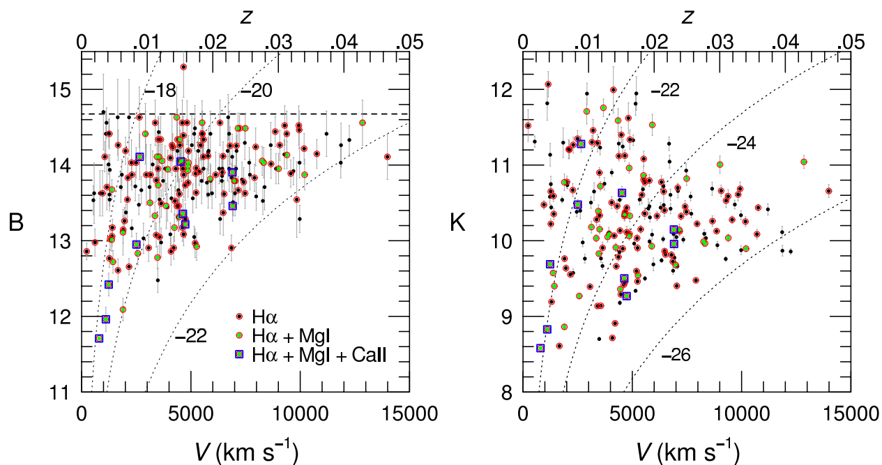
Fig. 10.— Hubble diagrams for the DMS in the B -band (left) and K -band (right). Sub-samples are marked according to the key: black points (Phase-A sample); red-encircled points ( \text{H}\alpha sample); green-cored points (Phase-B Mg Ib sample); blue-ensquared points (Phase-B Ca II sample). Objects in the Mg Ib sub-sample are also in the \text{H}\alpha sub-sample; objects in the Ca II sub-sample are also in Mg Ib and \text{H}\alpha sub-samples. Dotted lines of constant luminosity are marked. The B -band completeness limit of the UGC is delineated with a horizontal dashed line in the left panel. [COLOR]
