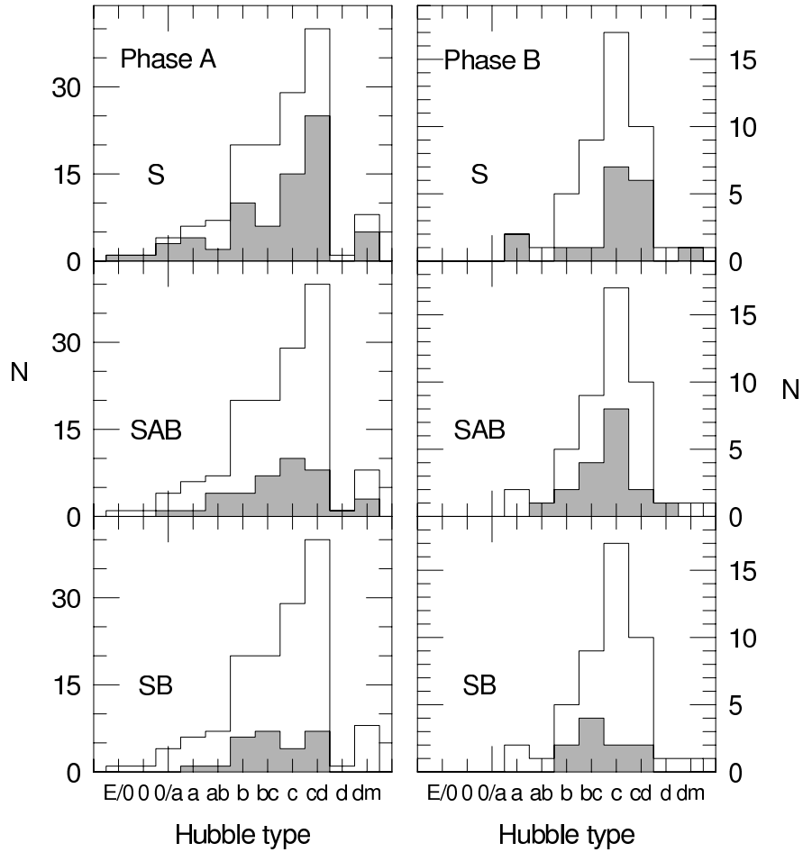
Fig. 8.— Distribution of Hubble types in Phase-A (left) and Phase-B (right) samples, broken down by un-barred (S), weakly-barred (SAB), and barred (SB) systems (grey histograms). Open histograms represent the total sample for all families; these are identical for the three panels in each column.
