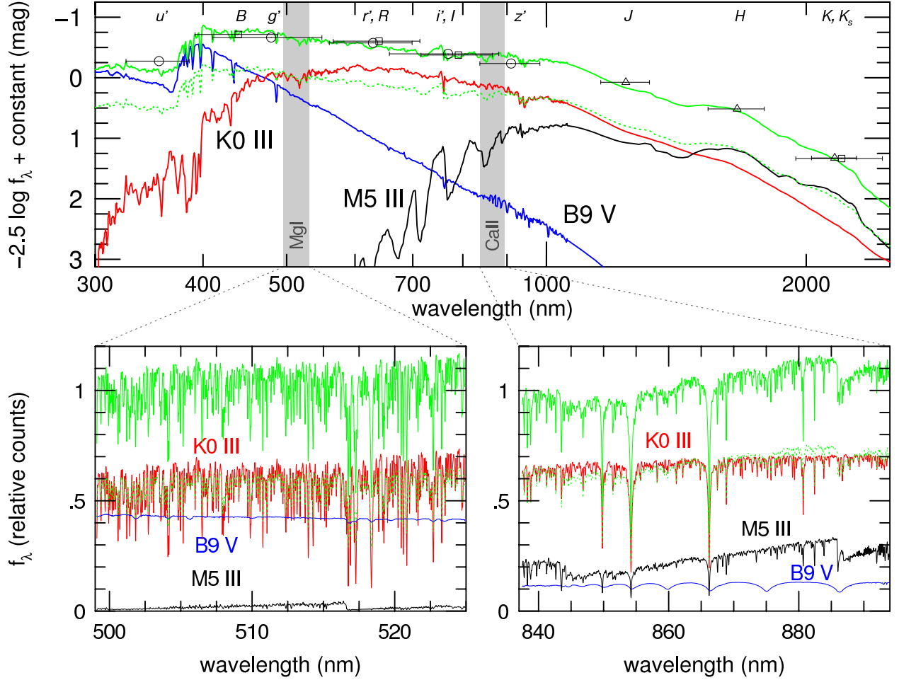
Fig. 7.— Three-star spectral-synthesis for UGC 6918, with integrated colors typical of galaxies in the DMS, at low-resolution (top panel) and high-resolution (bottom panels). Low-resolution spectra are from the compilation of Bruzual & Charlot (1993). High-resolution spectra are from our own echelle stellar-template library observed with SparsePak, and show the spectral regions used to measure \sigma_{\text{LOS}} in the DMS. Constraints on the spectral mix, described in the text, are based on broad-band photometry shown here as squares [ BVIK magnitudes from Verheijen (1997)], circles ( u'g'r'i'z' magnitudes based on our own photometric measurements on SDSS images), and triangles ( JHK_s measurements from 2MASS corrected as described in Appendix A). Individual star spectra are labeled (blue, red, black for B9 V, K0 III, and M5 III, respectively). In the Mg Ib-region and Ca II-region the flux ratios B9:K0:M5 are 0.42:0.56:0.02 and 0.12:0.65:0.23, respectively. Green solid curves show the combined spectrum using this mix. Green dotted curves are the combined spectrum renormalized to the dominant stellar spectrum in the Mg Ib region (top and bottom left panels) and Ca II region (bottom right panel), drawn to indicate the difference with a one-star template. [COLOR]
