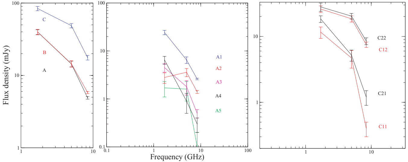
Figure 5. Left-hand panel: The radio spectra of lensed images A and B, and region C. Middle panel: The radio spectra of the components of lensed image A. Right-hand panel: The radio spectra of the components in region C. The data are taken from the global VLBI and HSA observations between 1.7 and 8.4 GHz.
