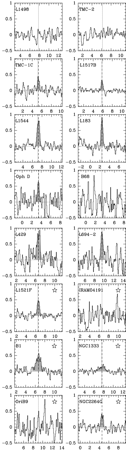
Fig. 1. ortho- \text{H}_2\text{D}^+ ( 1_{1,0}-1_{1,1} ) spectra toward the 16 sources of our sample. The units are main beam brightness temperature in K ( y -axis, assuming a unity filling factor) and velocity in \text{km s}^{-1} ( x -axis). A star in the top right indicates dense cores associated with protostellar objects. The vertical dotted line is the V_{\text{LSR}} velocity measured with \text{N}_2\text{H}^+ ( 1-0 ), whereas the vertical dashed line marks V_{\text{LSR}} as measured with the present \text{H}_2\text{D}^+ observations. Within the uncertainties, the two values are identical. Note that the strongest emission is present in the densest starless cores (L 1544, L 183, L 429, L 694-2) and in the star forming regions L 1521F, B 1, and NGC 2264G. Note also the large variation in linewidth among the various sources.
