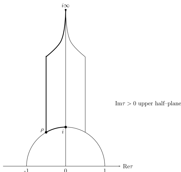
Figure 1: Fundamental domain of \text{PSL}(2, \mathbb{Z}) \backslash \text{PSL}(2, \mathbb{R}) / \text{SO}(2)
