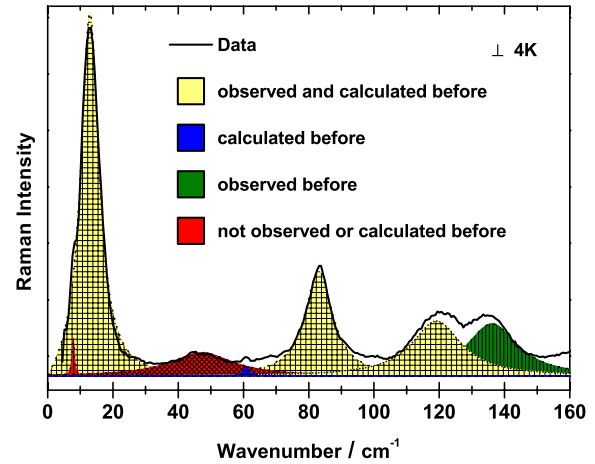
FIG. 6. (Color online) The low-wavenumber region of the perpendicular polarization Raman spectrum of \text{Tb}_2\text{Ti}_2\text{O}_7 at 4 K. A fitted Lorentzian centered at zero (Rayleigh line) is subtracted from the data for clarity. The crystal field levels (see Fig. 5) are indicated by the filled Lorentzian line shapes that were fitted to the data. A distinction has been made between CF levels that have been calculated and observed before (yellow), CF levels that have been calculated before but so far have not been observed (blue), CF levels that have been observed before but have not been calculated (green), and additional CF levels that are observed in this study using inelastic light scattering (red).
