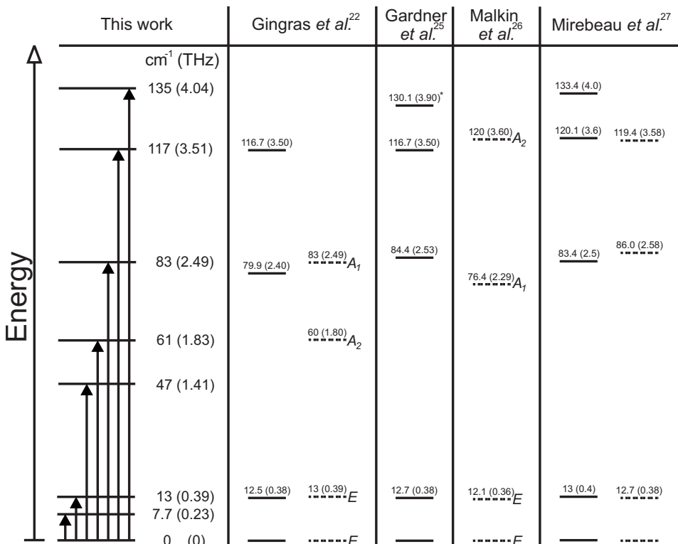
FIG. 5. Various CF energy-level schemes of the \text{Tb}^{3+} ion in \text{Tb}_2\text{Ti}_2\text{O}_7 . Solid lines depict CF levels that have been observed experimentally, while dotted lines represent CF levels as calculated using CF calculations. Numbers indicate CF level energies in \text{cm}^{-1} (THz); symbols in italics indicate symmetries of corresponding levels. Solid arrows indicate all CF excitations observed in the low-temperature Raman spectrum of \text{Tb}_2\text{Ti}_2\text{O}_7 (see Fig. 6).
