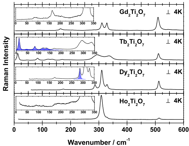
FIG. 4. (Color online) Low-temperature spectra for all R_2\text{Ti}_2\text{O}_7 as measured in perpendicular polarization configuration. The spectra are normalized to the total integrated intensity of the spectra. The insets show respective zooms on the lower-wavenumber regions of the spectra, where the excitations identified as CF levels of the rare earth ions are indicated by dotted blue Lorentzian peaks. \text{Gd}_2\text{Ti}_2\text{O}_7 shows only phononic modes and can be regarded as the lattice template. \text{Tb}_2\text{Ti}_2\text{O}_7 and \text{Dy}_2\text{Ti}_2\text{O}_7 show additional CF modes, while \text{Ho}_2\text{Ti}_2\text{O}_7 shows again only lattice excitations. A fitted Lorentzian centered at zero (Rayleigh line) is subtracted from the \text{Tb}_2\text{Ti}_2\text{O}_7 data for clarity.
