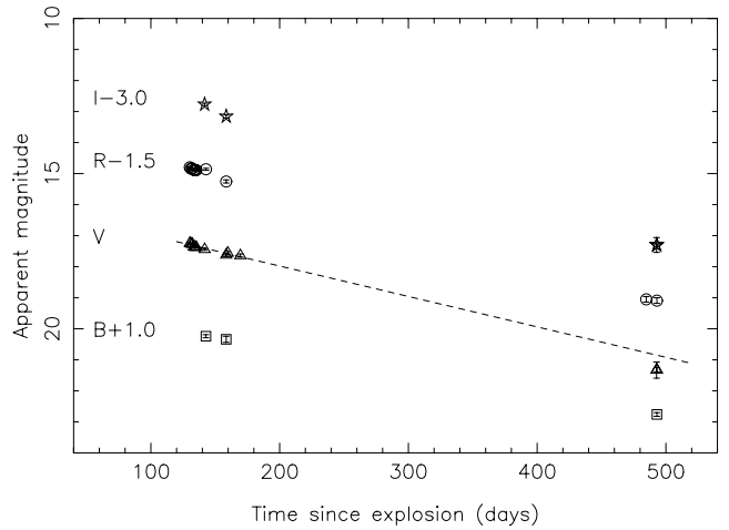
Figure 11. BVRI nebular and late-time photometry of SN 2003gd with a linear fit of the earlier nebular data, in the V band, shown with a dashed line. The late-time photometry, in the V band, is lower than what we would expect from the earlier photometry.
