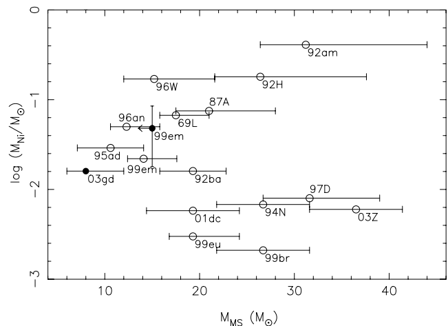
Figure 22. Reproduction of fig. 1 (right) of Zampieri et al. (2004) showing the bimodal distribution of SNe II-P, in the M_{\text{Ni}}/M_{\text{MS}} plane, from their model. The open circles show theoretical data from the semi-empirical model of Zampieri et al. (2003), where M_{\text{MS}} is estimated from the ejected envelope mass. The filled circles show observational data for SNe 2003gd and 1999em, where M_{\text{Ni}} is estimated from the light curve and M_{\text{MS}}^{199\text{em}} is an upper mass limit only (Smartt et al. 2002a). SN 2003gd inhabits the lower end of the normal Type II-P branch.
