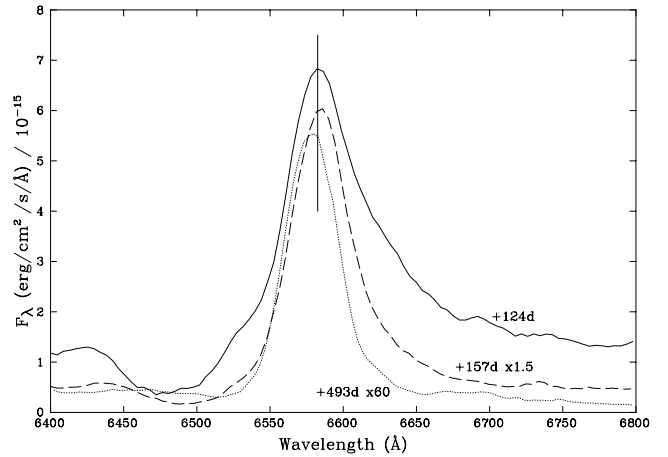
Figure 14. \text{H}\alpha profiles of SN 2003gd from 124, 157 and 493 d post-explosion. The vertical line marks the maximum of the \text{H}\alpha emission from the earliest spectrum. The peak of the \text{H}\alpha emission from 157 d shows a slight redshift of the peak, but the latest spectrum clearly shows a shift to the blue.
