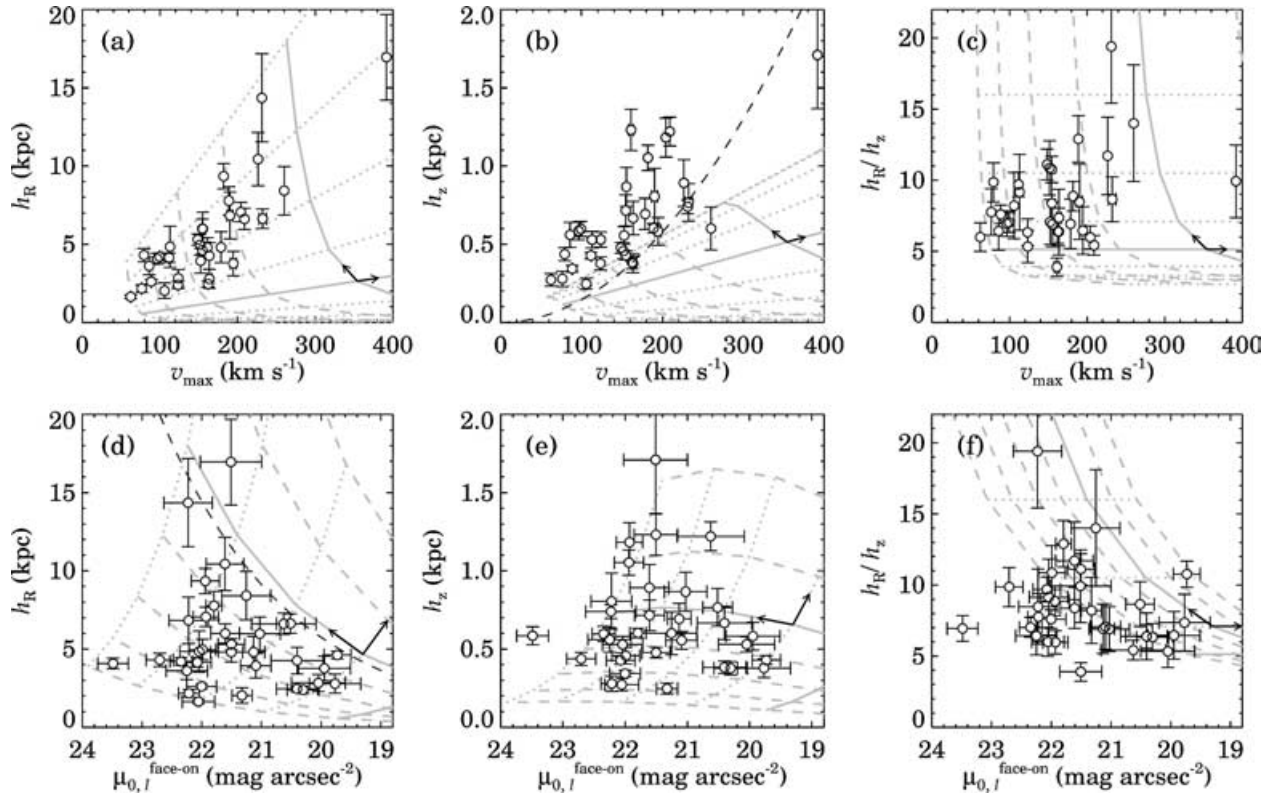
Figure 1. The disc scalelength, scaleheight and flattening as functions of maximum rotational velocity (a)–(c) and face-on central surface brightness (d)–(f). The black dashed line in (d) is the relation for exponential discs with luminosity L_* = 4 \times 10^{10} L_{\odot, l} . In each panel the grey lines show the collapse model for disc galaxy formation, the dashed lines connect models of the same total mass [ \log_{10}(M_{\text{tot}}) = 10\text{--}13 in steps of 0.5, and the solid line at \log_{10}(M_{\text{tot}}) = 12 ] and dotted lines connect models with the same spin parameter (logarithmically spaced, separated by factors of 0.2 dex, solid line at \lambda = 0.06 ). Arrows indicate the direction of increasing M_{\text{tot}} and \lambda .
