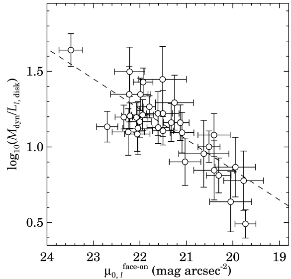
Figure 5. The dynamical mass to disc luminosity ratio versus the face-on central surface brightness of the disc. The dashed line indicates an M_{\text{dyn}}/L \propto \mu_{0, I}^{-1/2} relation, arbitrarily shifted in zero-point to match the observed relation.
