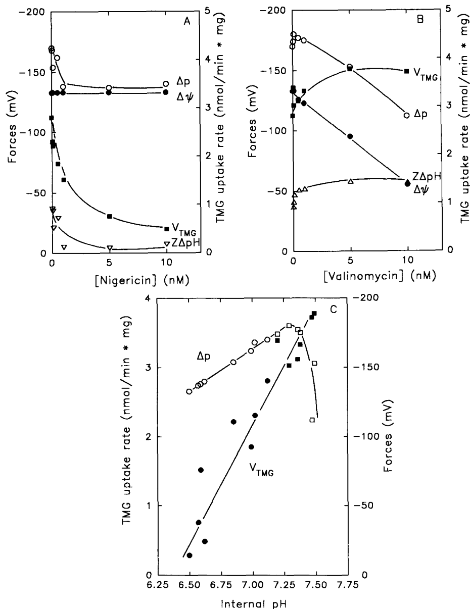
FIG. 3. Effect of increasing concentrations of ionophores on TMG uptake and the magnitude of the components of the \Delta p , and the internal pH dependence of the initial rate of TMG uptake. Fused membranes were resuspended in HMP buffer, pH 6.5, and energized by ascorbate-TMPD-cytochrome c oxidation. Increasing concentrations nigericin (panel A) and valinomycin (panel B) were added. Conditions were similar to those described in the legend to Fig. 1 except that the final protein concentration was 0.24 mg/ml. The initial rate of TMG uptake was estimated from the amount of label accumulated over 5 s, and the magnitudes of the components of the \Delta p were estimated as described. Panel C, The dependence of the initial rate of TMG uptake on the internal pH (data were taken from panels A and B). For comparison the magnitude of the \Delta p is also shown.
