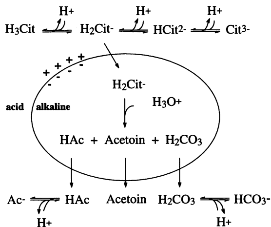
FIG. 8. Proposed model for PMF generation by citrate metabolism in L. oenos . H_3Cit , citric acid; HAc , acetic acid.
