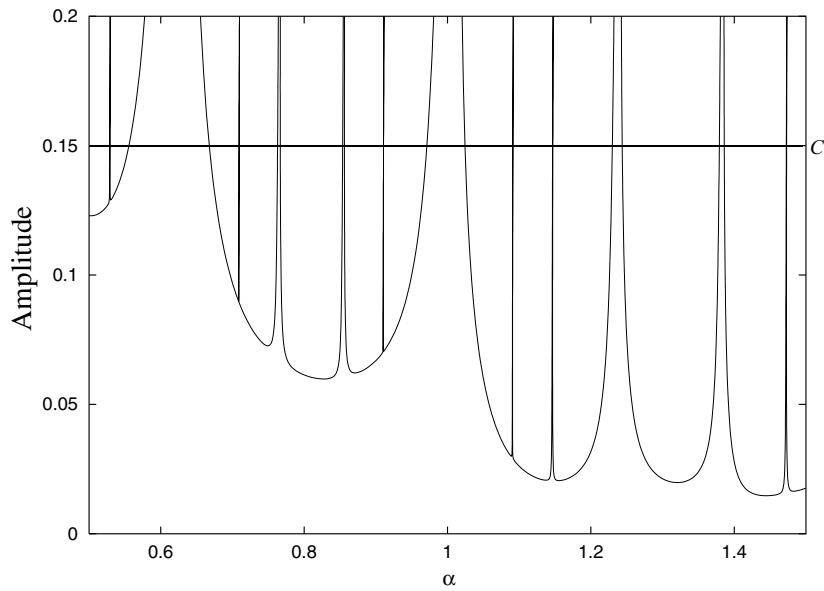
Figure 1. Response diagram of (1) and (2). Shown are the parameter \alpha on the horizontal axis, against the L^2 norm of the response solution on the vertical axis. Classical KAM-theory can only prove the existence of invariant tori whose L^2 norm is below some bound c , which is of the same order O(\varepsilon) as the forcing, as \varepsilon \rightarrow 0 . Moreover the normal dynamics of these invariant tori should be elliptic, which fails to be the case for 1 : 2 resonances (the corresponding gaps are not shown in this figure).
