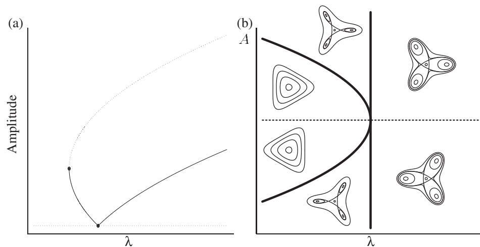
Figure 7. (a) Response diagram for the case \ell = 3 : dotted lines indicate elliptic equilibria, solid lines correspond to hyperbolic equilibria. (b) Structurally stable phase portraits in a (\lambda, A) -bifurcation diagram.
