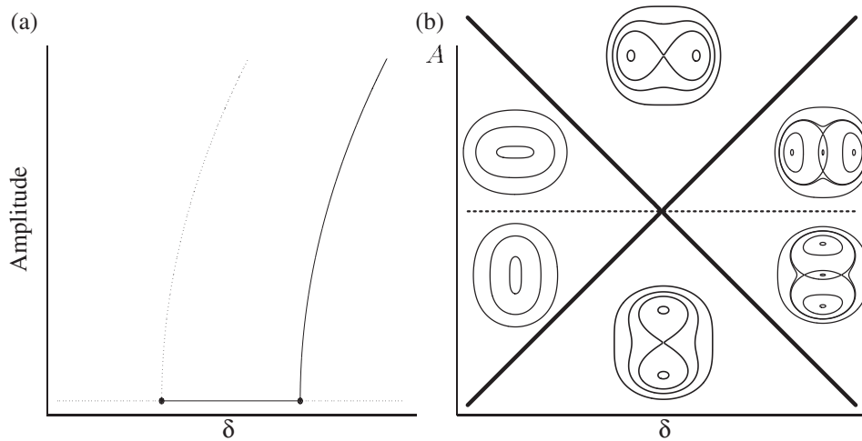
Figure 6. (a) Response diagram for the case \ell = 2 : dotted lines indicate elliptic equilibria, solid lines correspond to hyperbolic equilibria. (b) Structurally stable phase portraits in a (\delta, A) -bifurcation diagram.
