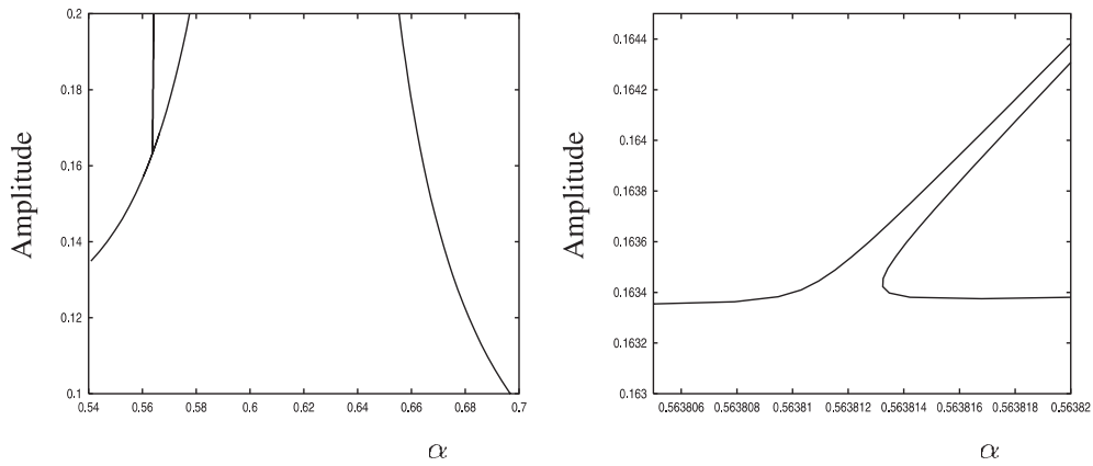
Figure 2. Two more response diagrams associated with the 1 : 1 normal-internal resonance. The left plot shows the big resonance for \alpha near the golden number -\frac{1}{2} + \frac{1}{2}\sqrt{5} = 0.618\dots , and the right plot is a magnification of the ‘secondary’ gap that appears in the left plot.
