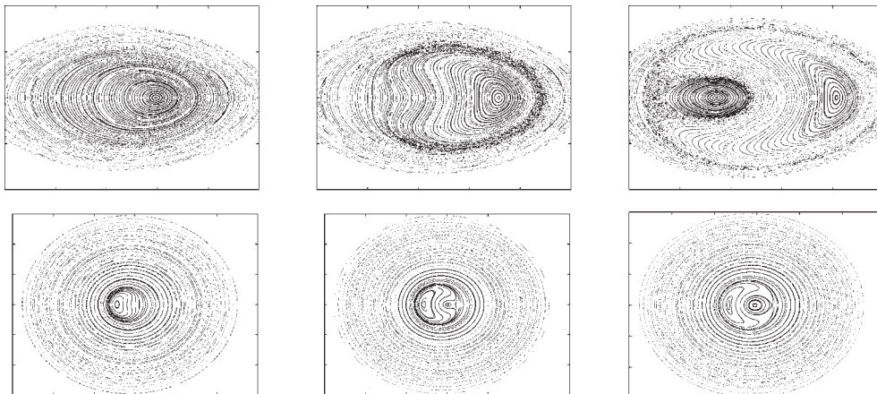
Figure 3. Six phase portraits associated with the 1 : 1-resonance, the first three for \alpha \approx -\frac{1}{2} + \frac{1}{2}\sqrt{5} , and the other three for ‘a gap within that gap’ ( \alpha \approx 0.563\,813 , see figure 2, left).
