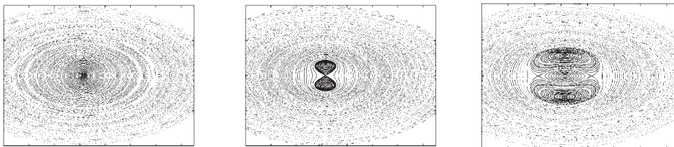
Figure 4. Three phase portraits associated with a 1 : 2-resonance, for -3(-\frac{1}{2} + \frac{1}{2}\sqrt{5}) + 2\alpha \approx 0 .
