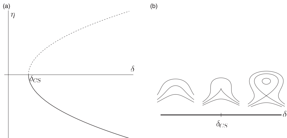
Figure 9. (a) Bifurcation diagram of the centre-saddle bifurcation where \delta is the bifurcation parameter and \eta is some well-chosen auxiliary variable. (b) Phase portraits before, at and after the bifurcation.
