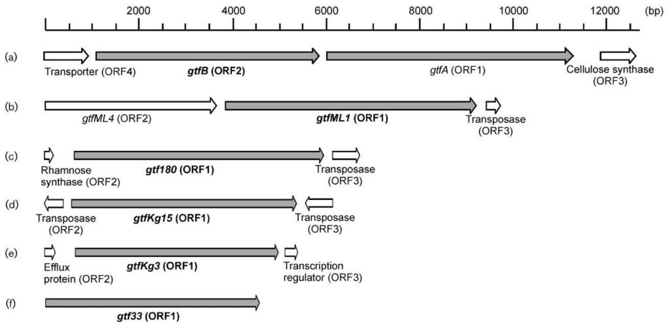
Fig. 1. Overview of the size and organization of DNA fragments, isolated by iPCR, carrying the different gtf genes and surrounding regions from six different Lactobacillus strains characterized in this study (shown in bold type): (a) gtfA (characterized previously, Kralj et al. , 2002) and gtfB from Lactobacillus reuteri 121; (b) gtfML1 and (partly) gtfML4 from Lactobacillus reuteri ML1; (c) gtf180 from Lactobacillus reuteri 180; (d) gtfKg15 from Lactobacillus sakei Kg15; (e) gtfKg3 from Lactobacillus fermentum Kg3; (f) gtf33 from Lactobacillus parabuchneri 33. Partial ORFs are indicated with open arrows.
