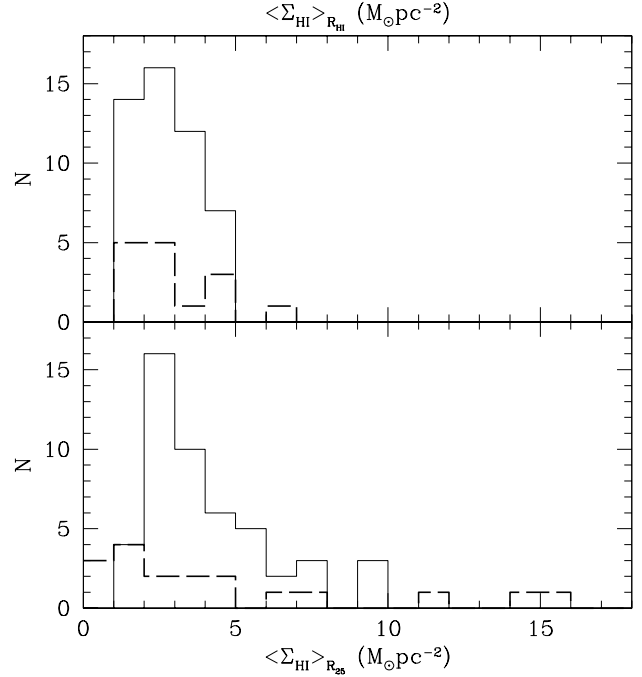
Fig. 7. The distribution of average HI surface density within the 1 M_{\odot} \text{pc}^{-2} isophote ( top ) and within the optical diameter ( bottom ). The solid line indicates all galaxies with type Sa and Sab, the dashed line indicates the S0's.
