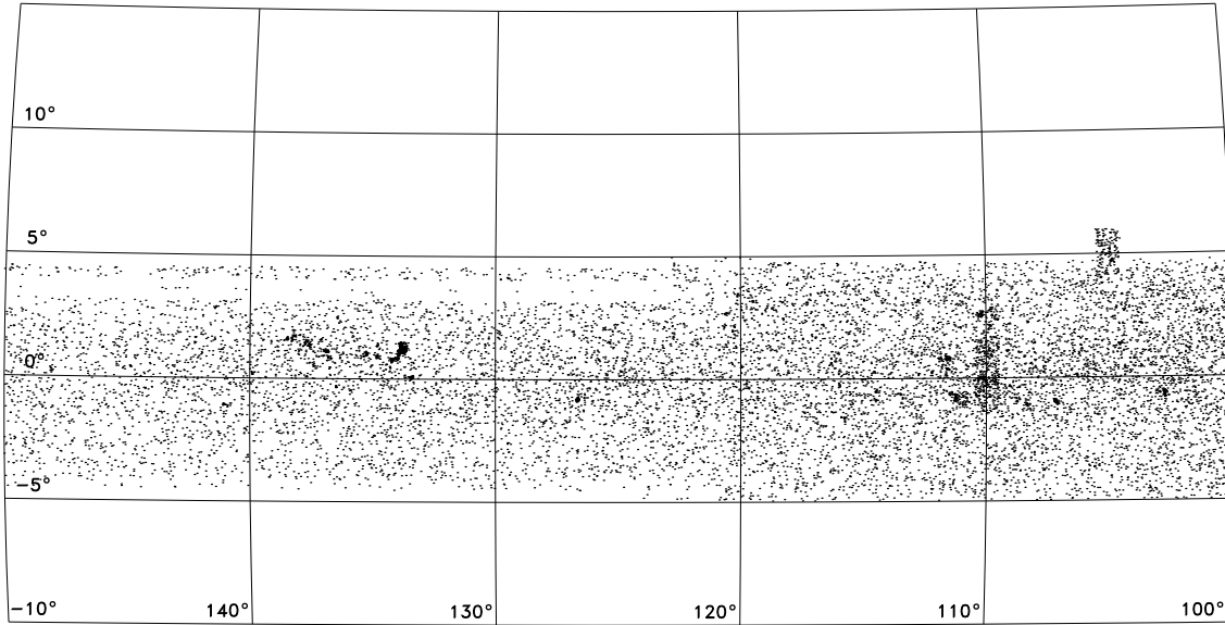
FIG. 2.— MSX point sources in the outer Galaxy. All sources listed in the Point Source Catalog (Egan et al. 2003) are plotted. Overdensities near the position of Complex H ( l = 131^\circ, b = 1^\circ ; see Figure 1) are visible, but they can all be identified with nearby Milky Way H II regions.
