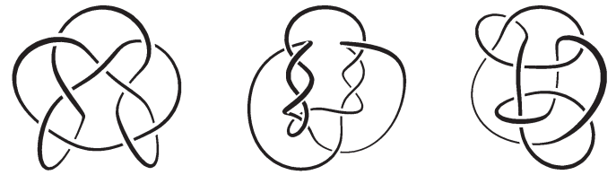
Fig. 16. Visualizations of simple mathematical shapes from knot theory.
