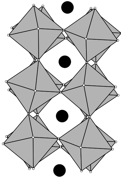
Figure 1. A general perovskite structure consisting of corner sharing octahedra. The octahedra consist of oxygen ions at the corners and Mn ions at the centre. The R ions occupy the voids between the octahedra.
