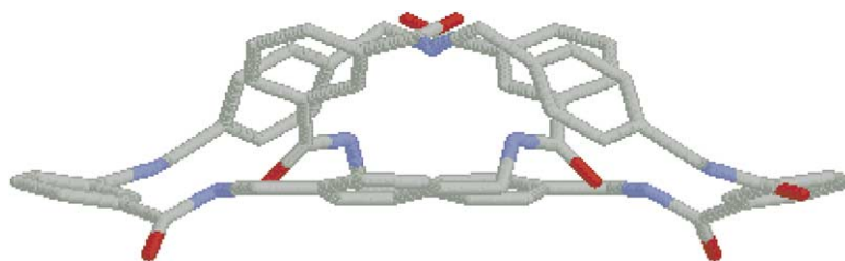
Fig. 4. Structure of a chemisorbed catenane on Au(1 1 1) as determined by MM3 calculations. The grey parts indicate carbon atoms, red parts correspond to oxygen atoms and blue parts represent nitrogen atoms, hydrogen atoms are not shown.
