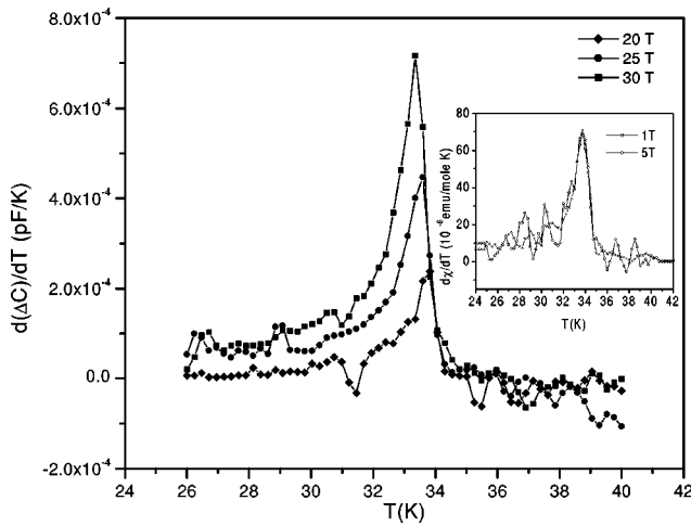
FIG. 2. Derivative of the unscaled capacitance readings (proportional to magnetization) with respect to temperature for the sample shown in Fig. 1 located at field center. Inset shows low field SQUID magnetization measurements.
