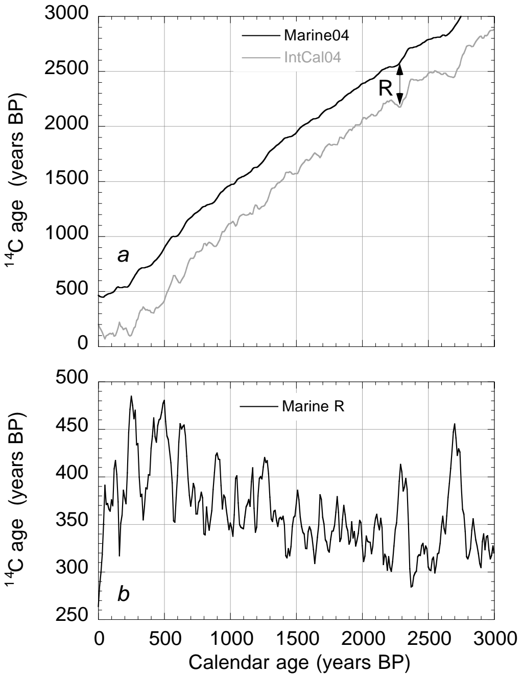
Figure 4 Global marine reservoir age “ R ” for the past 3000 yr. Atmospheric ^{14}\text{C} changes quickly following production spikes, but is muted in the ocean mixed layer. As a result, R calculated by the difference between IntCal04 and box diffusion model output (curve a) shows large variability (curve b). Beyond 10.5 cal kyr BP, when the Marine04 curve relies entirely on marine ^{14}\text{C} data sets, the global reservoir R is held constant at 405 yr (see Figure 2).
