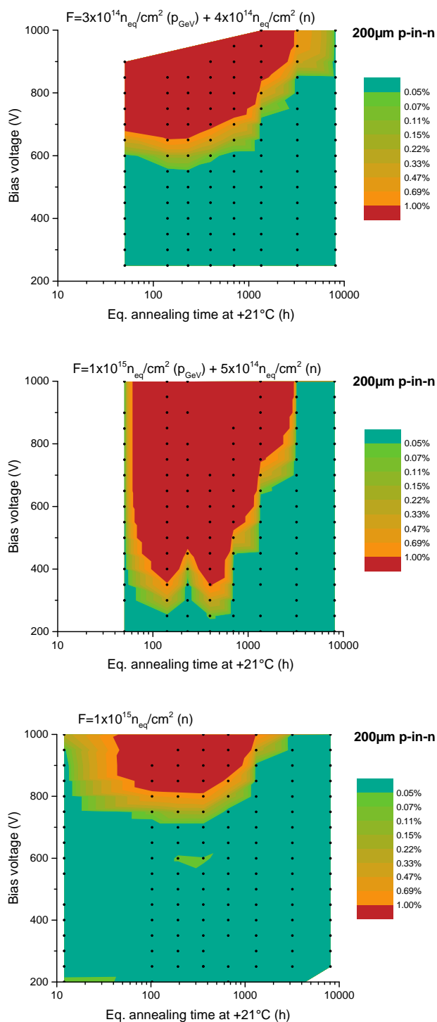
Figure 11. Measured occupancy of misidentified hits generated by non-Gaussian noise. These examples are for p-in-n sensors with 200 \mu\text{m} active and physical thickness irradiated to 7 \times 10^{14} n_{\text{eq}}/\text{cm}^2 (top) and 1.5 \times 10^{15} n_{\text{eq}}/\text{cm}^2 (center) with mixed particles and to 1 \times 10^{15} n_{\text{eq}}/\text{cm}^2 with only neutrons (bottom). The black dots represent the data points and the color code interpolates between them. White areas lie outside the measurement range.
